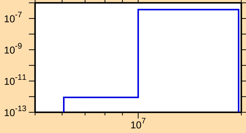
\sigma vs. E for ^{193}\text{Pb}(n,\text{He}3)
