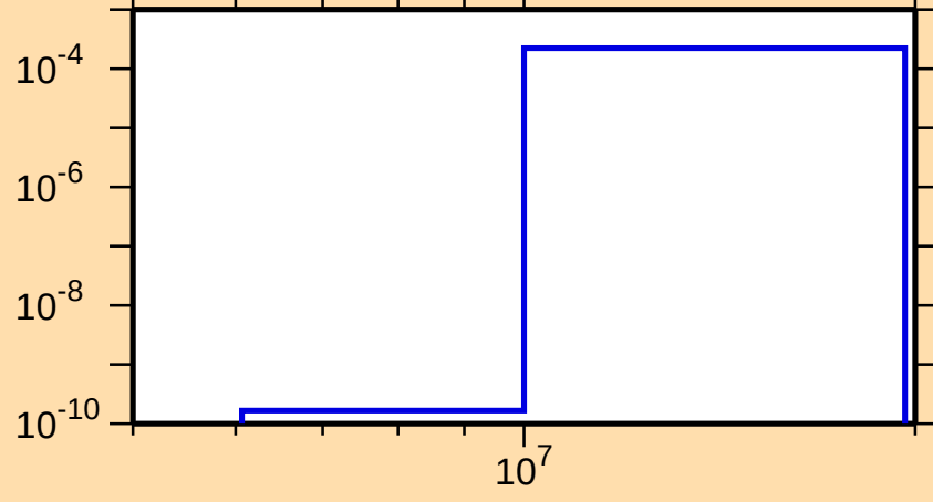
\sigma vs. E for ^{193}\text{Pb}(n,t)
