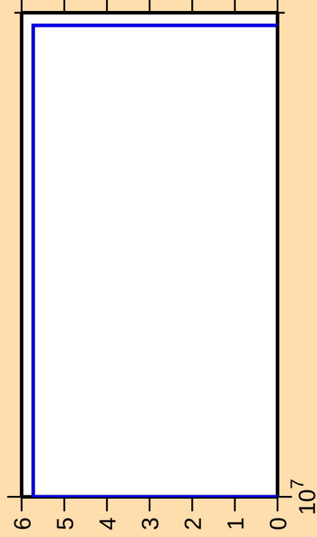
\Delta\sigma/\sigma vs. E for ^{193}\text{Pb}(n,nt)
