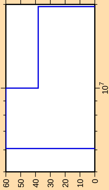
\Delta\sigma/\sigma vs. E for ^{193}\text{Pb}(n,2n)
