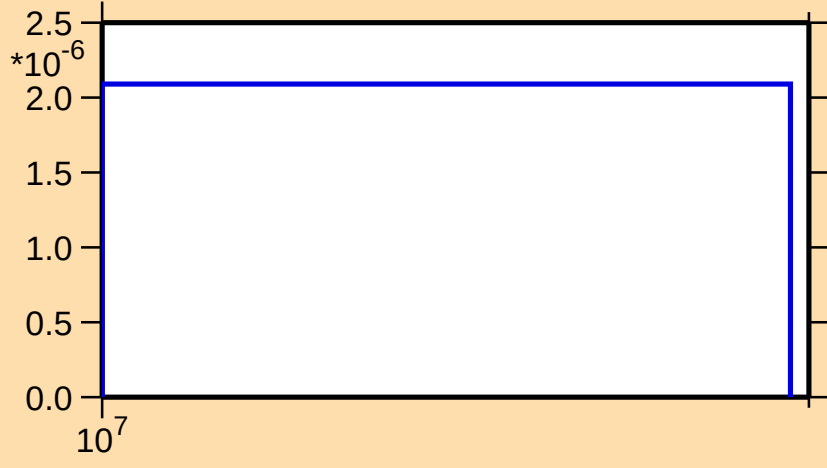
\sigma vs. E for ^{193}\text{Pb}(n,2np)
