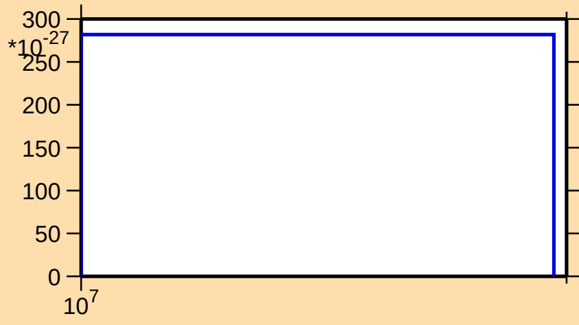
\sigma vs. E for ^{193}\text{Pb}(\text{mt } 11)
