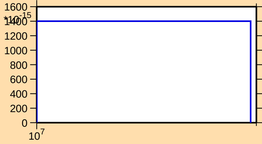
\sigma vs. E for ^{193}\text{Pb}(\text{mt } 34)
