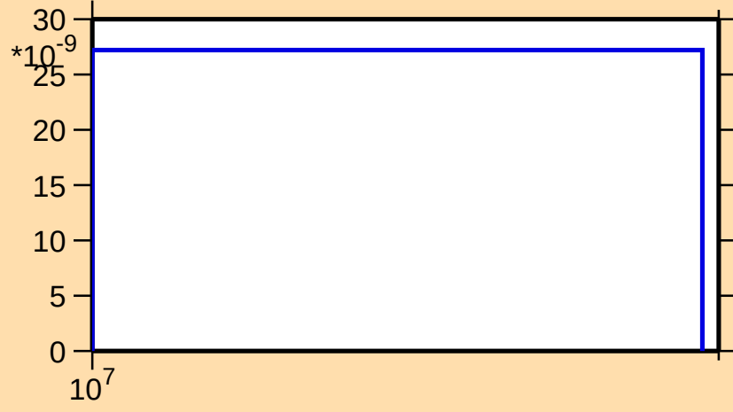
\sigma vs. E for ^{193}\text{Pb}(n,\text{nd})
