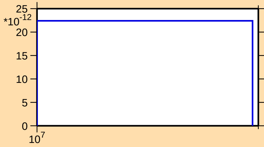
\sigma vs. E for ^{193}\text{Pb}(\text{mt } 45)
