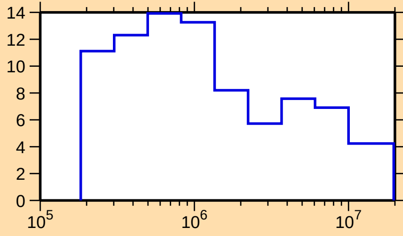
\Delta\sigma/\sigma vs. E for ^{193}\text{Pb}(n,\text{tot.})
