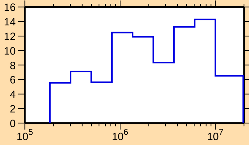
\Delta\sigma/\sigma vs. E for ^{193}\text{Pb}(n,\text{el.})
