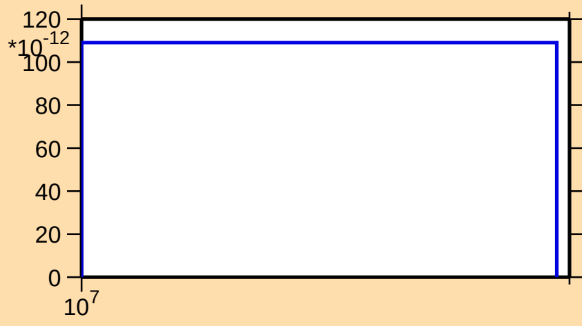
\sigma vs. E for ^{193}\text{Pb}(n,\text{pd})
