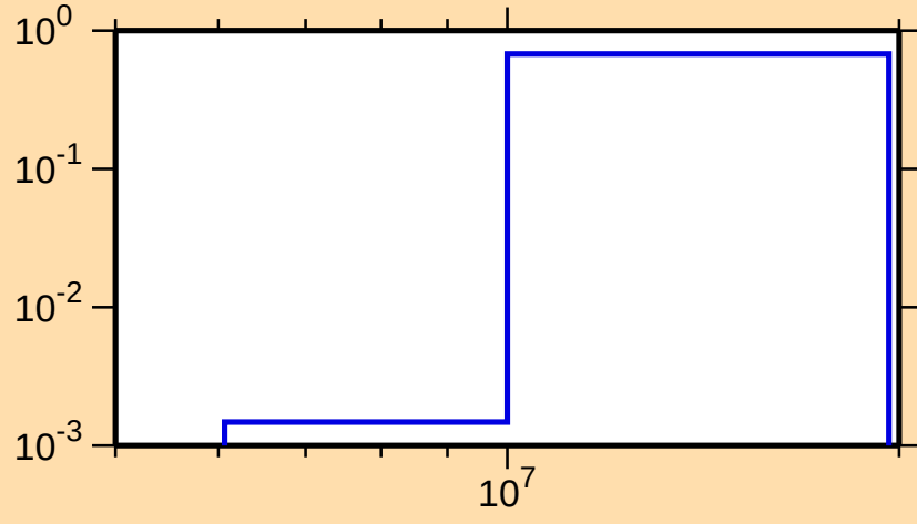
\sigma vs. E for ^{193}\text{Pb}(n,2n)
