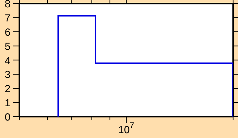
\Delta\sigma/\sigma vs. E for ^{193}\text{Pb}(n,\text{tot.})
