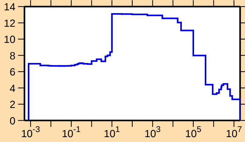
\sigma vs. E for ^{193}\text{Pb}(n,\text{el.})
