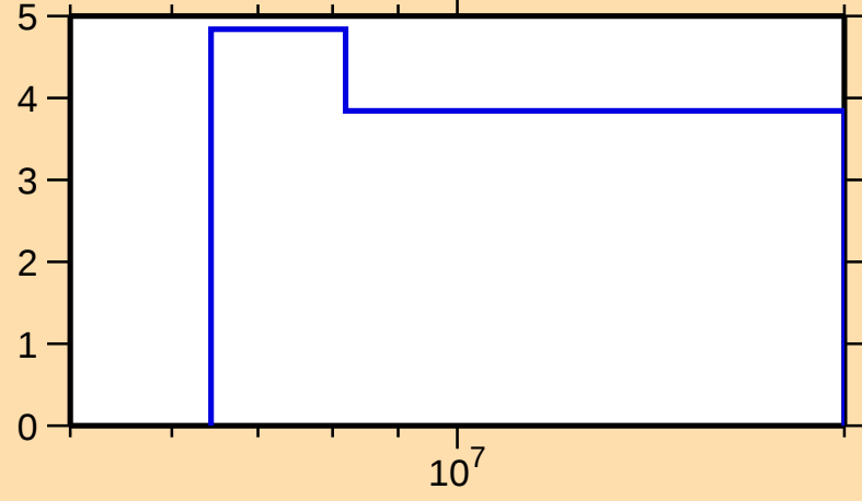
\Delta\sigma/\sigma vs. E for ^{193}\text{Pb}(n,\text{nonel.})
