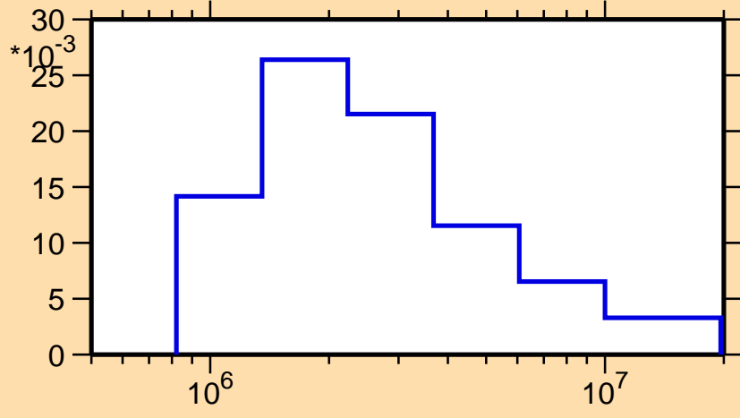
\sigma vs. E for ^{195}\text{Pb}(n,n_4)
