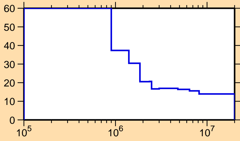
\Delta\sigma/\sigma vs. E for ^{195}\text{Pb}(n,\text{nonel.})
