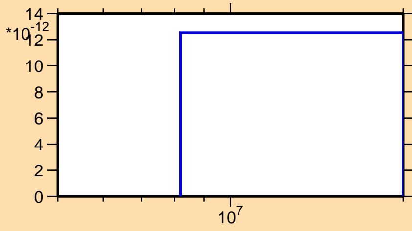
\sigma vs. E for ^{195}\text{Pb}(n,\text{pd})
