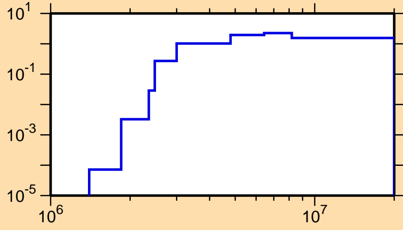
\sigma vs. E for ^{195}\text{Pb}(n,n\text{cont.})
