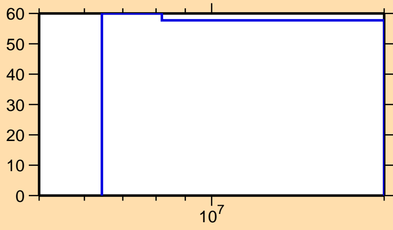
\Delta\sigma/\sigma vs. E for ^{195}\text{Pb}(n,2n)
