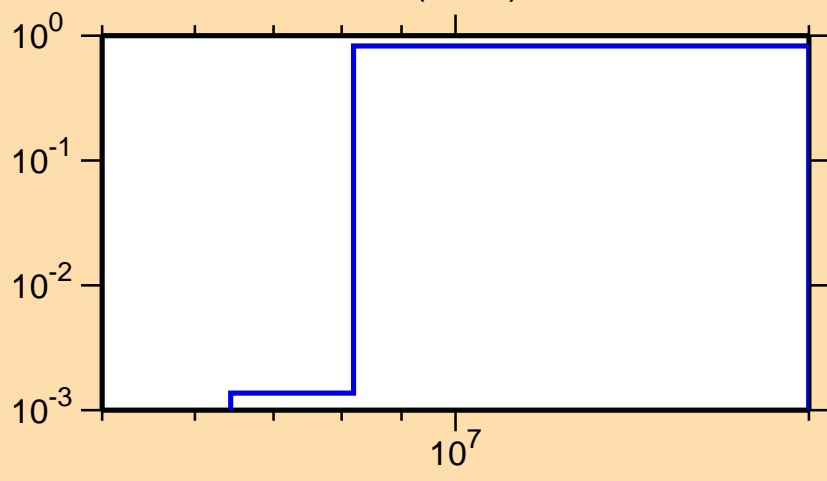
\sigma vs. E for ^{195}\text{Pb}(n,2n)
