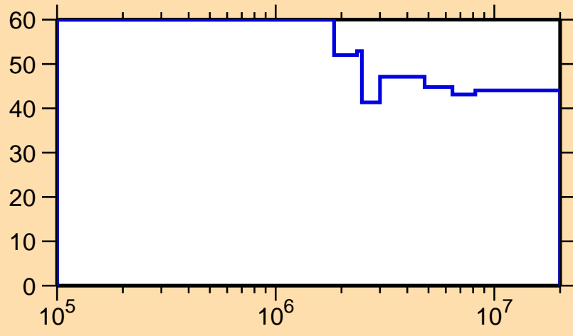
\Delta\sigma/\sigma vs. E for ^{195}\text{Pb}(n,n_1)
