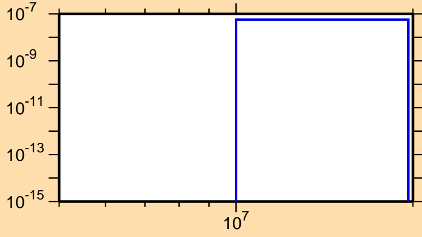
\sigma vs. E for ^{195}\text{Pb}(n,2n\alpha)
