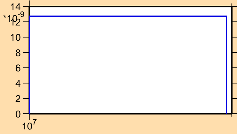
\sigma vs. E for ^{195}\text{Pb}(n,\text{nd})
