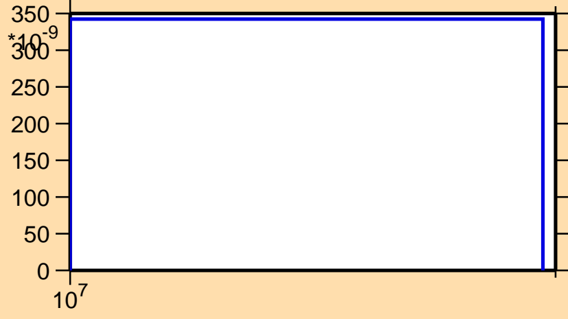
\sigma vs. E for ^{195}\text{Pb}(n,2np)
