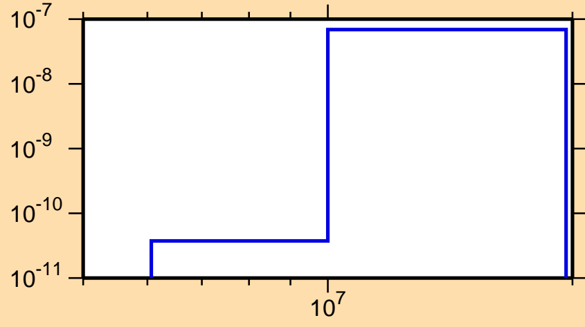
\sigma vs. E for ^{195}\text{Pb}(n,p\alpha)
