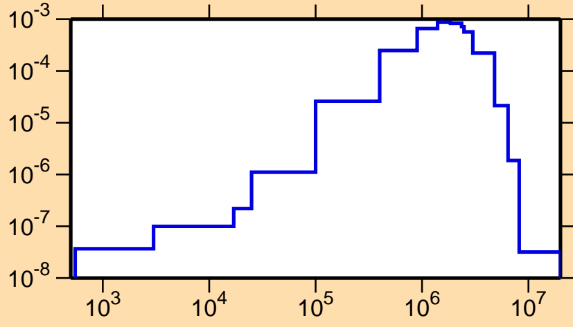
\sigma vs. E for ^{195}\text{Pb}(n,n_1)
