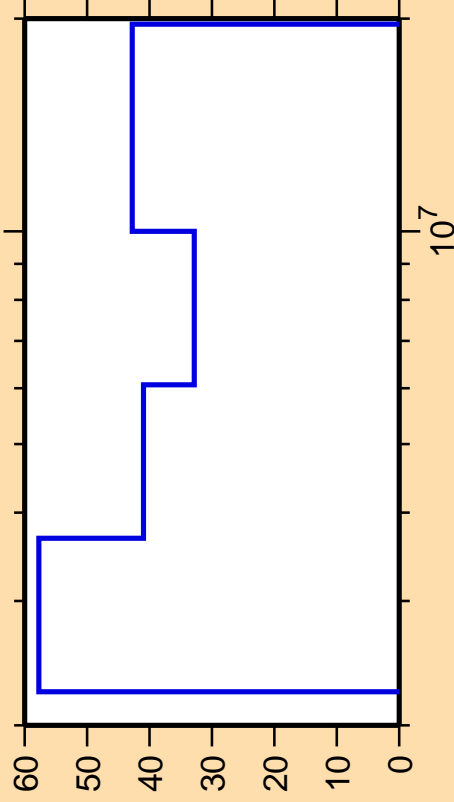
\Delta\sigma/\sigma vs. E for ^{196}\text{Pb}(n,n\text{cont.})
