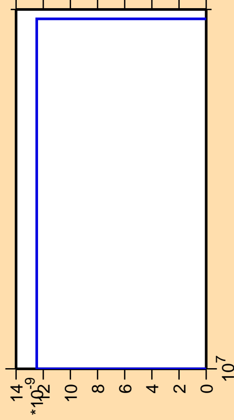
\Delta\sigma/\sigma vs. E for ^{196}\text{Pb} (mt 11)
