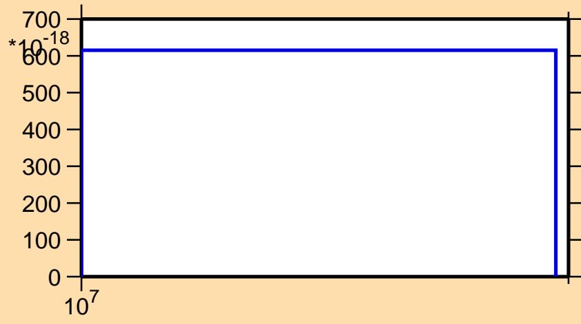
\sigma vs. E for ^{196}\text{Pb} (mt 34)
