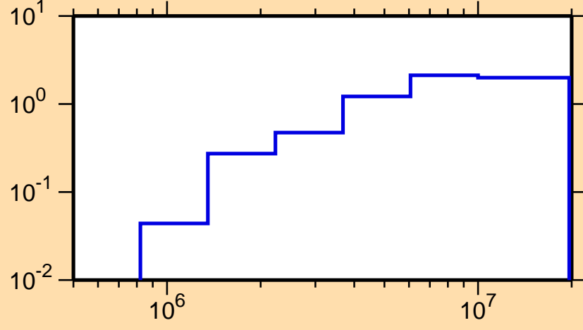
\sigma vs. E for ^{196}\text{Pb}(n,\text{inel.})
