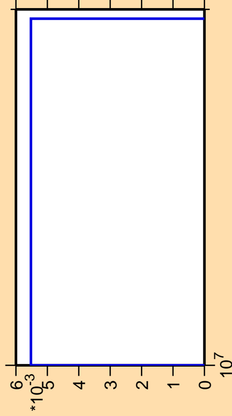
\Delta\sigma/\sigma vs. E for ^{196}\text{Pb} (mt 34)
