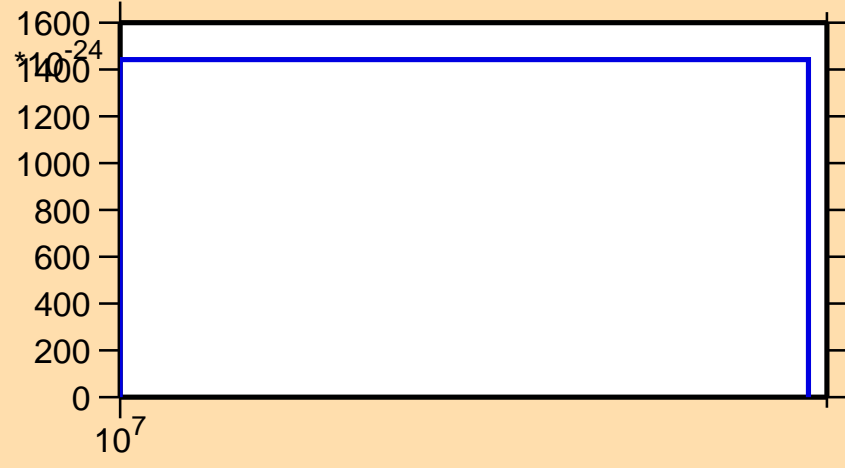
\sigma vs. E for ^{196}\text{Pb} (mt 11)
