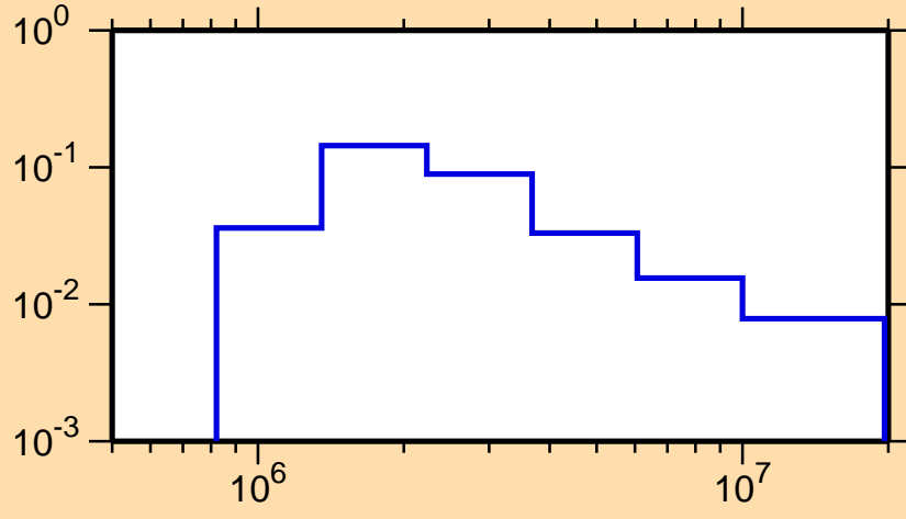
\sigma vs. E for ^{196}\text{Pb}(n,n_1)
