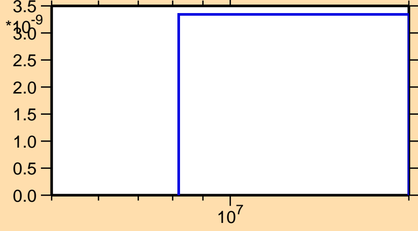
\sigma vs. E for ^{196}\text{Pb}(n,2np)
