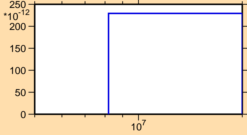
\sigma vs. E for ^{196}\text{Pb}(n,nd)
