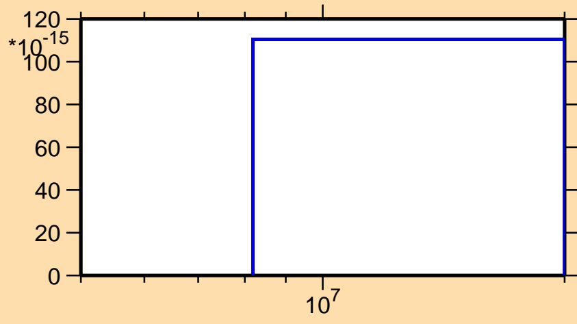
\sigma vs. E for ^{196}\text{Pb}(\text{mt } 45)
