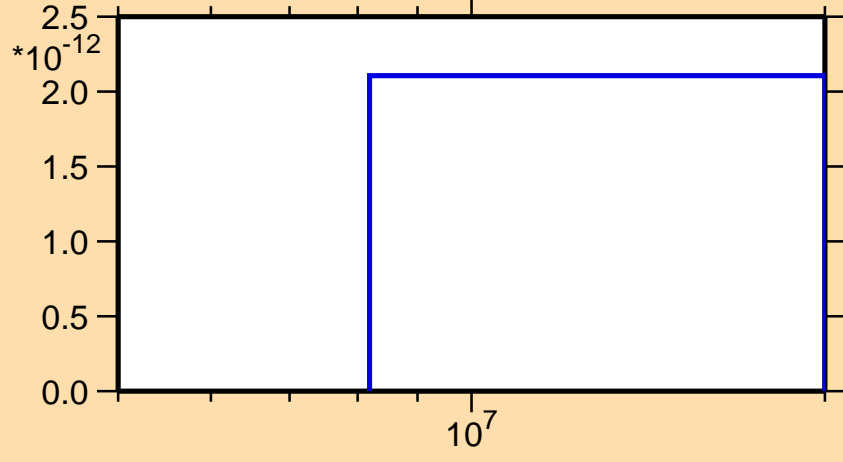
\sigma vs. E for ^{196}\text{Pb}(n,pd)
