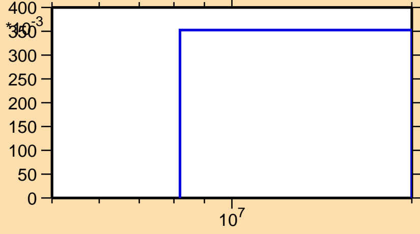
\sigma vs. E for ^{196}\text{Pb}(n,2n)
