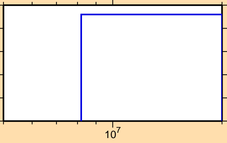
\sigma vs. E for ^{196}\text{Pb}(\text{mt117})
