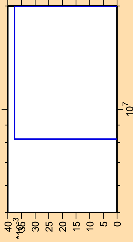
\Delta\sigma/\sigma vs. E for ^{196}\text{Pb}(\text{mt117})
