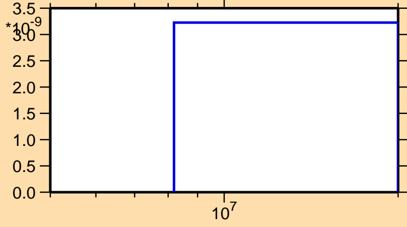
\sigma vs. E for ^{196}\text{Pb}(n,\text{He}3)
