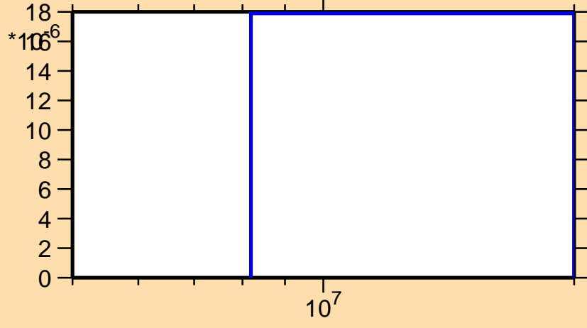
\sigma vs. E for ^{196}\text{Pb}(n,t)
