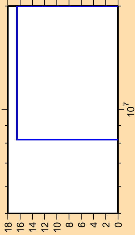
\Delta\sigma/\sigma vs. E for ^{196}\text{Pb}(n,pd)
