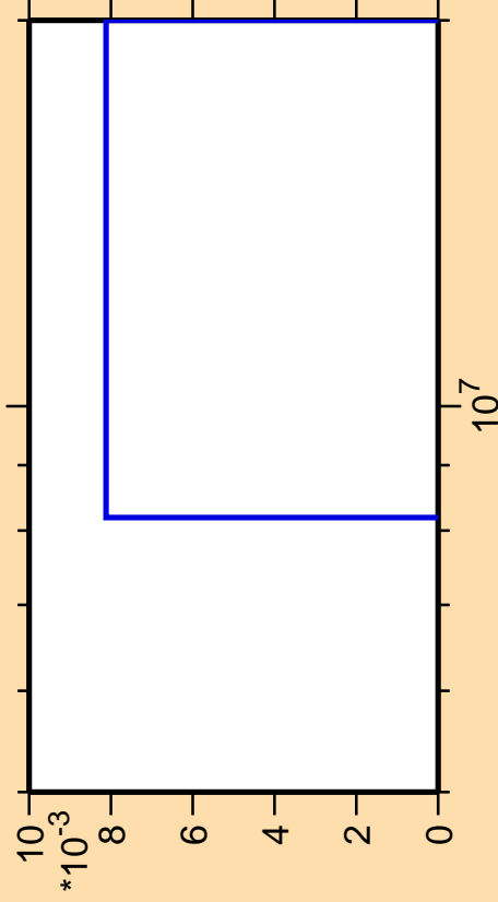
\Delta\sigma/\sigma vs. E for ^{196}\text{Pb}(n,\text{pt})
