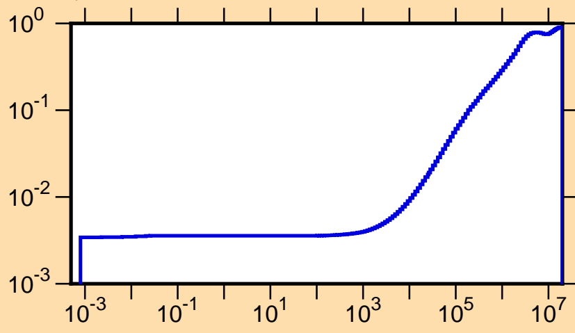
\mu vs. E for ^{197}\text{Pb}(\text{mt251})
