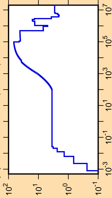
\Delta\mu/\mu vs. E for ^{197}\text{Pb}(\text{mt251})
