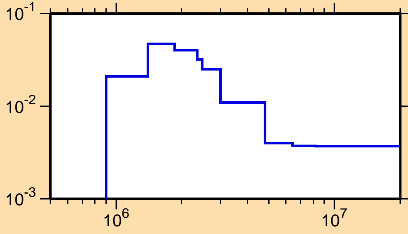
\sigma vs. E for ^{197}\text{Pb}(n,n_4)
