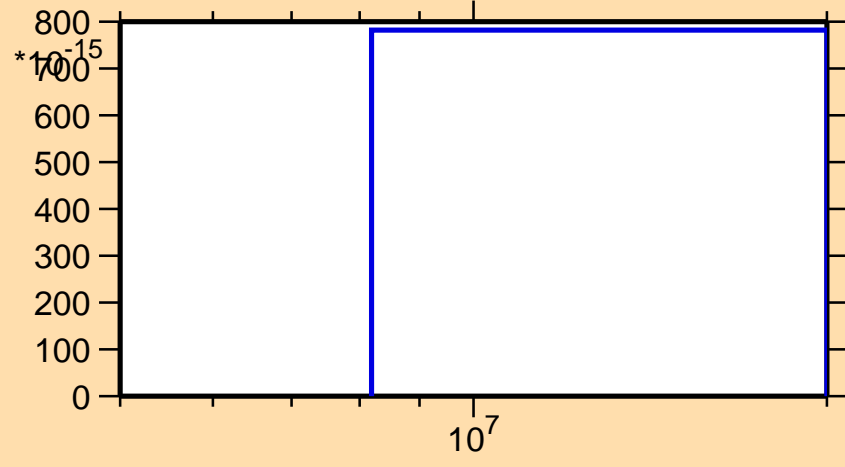
\sigma vs. E for ^{197}\text{Pb}(n,pd)
