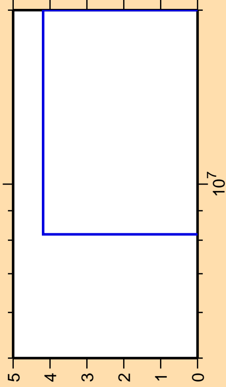
\Delta\sigma/\sigma vs. E for ^{197}\text{Pb}(n,pd)
