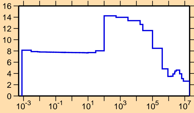
\sigma vs. E for ^{197}\text{Pb}(n,\text{el.})
