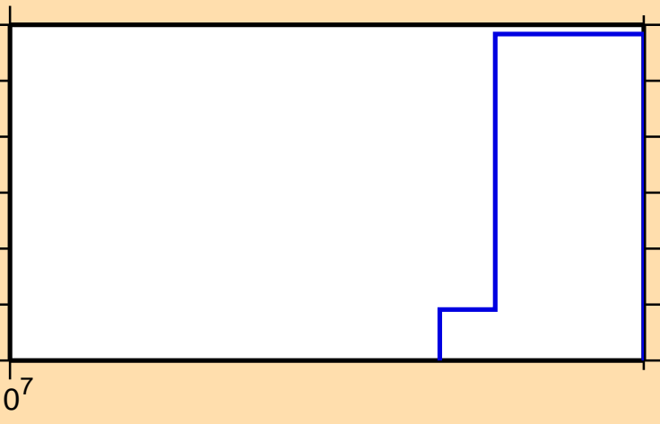
\sigma vs. E for ^{197}\text{Pb}(n,3n)
