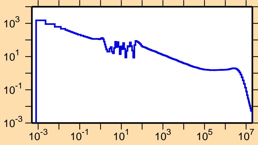
\sigma vs. E for ^{197}\text{Pb}(n,\gamma)
