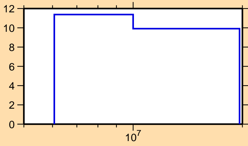
\Delta\sigma/\sigma vs. E for ^{197}\text{Pb}(n,\text{tot.})
