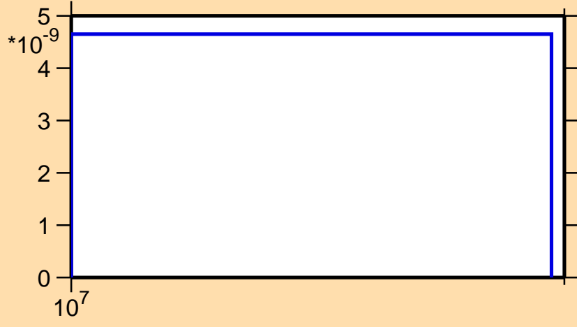
\sigma vs. E for ^{197}\text{Pb}(n,\text{nd})
