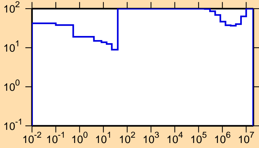
\Delta\sigma/\sigma vs. E for ^{197}\text{Pb}(n,\gamma)
