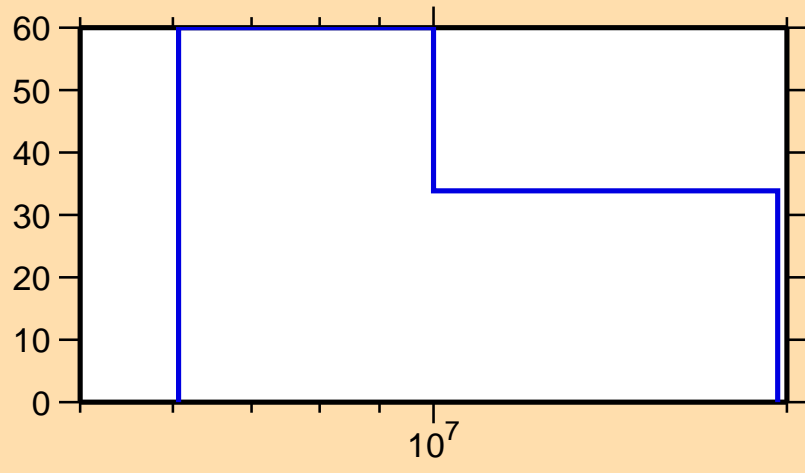
\Delta\sigma/\sigma vs. E for ^{197}\text{Pb}(n,2n)
