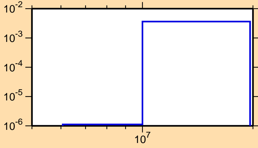
\sigma vs. E for ^{197}\text{Pb}(n,np)
