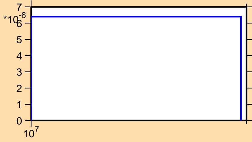
\sigma vs. E for ^{197}\text{Pb}(n,3n)
