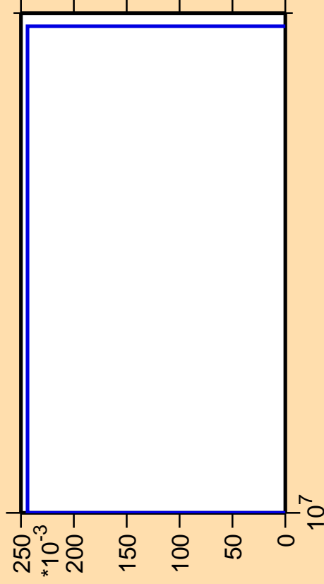
\Delta\sigma/\sigma vs. E for ^{197}\text{Pb}(n,\text{pt})
