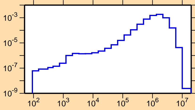
\sigma vs. E for ^{197}\text{Pb}(n,n_1)
