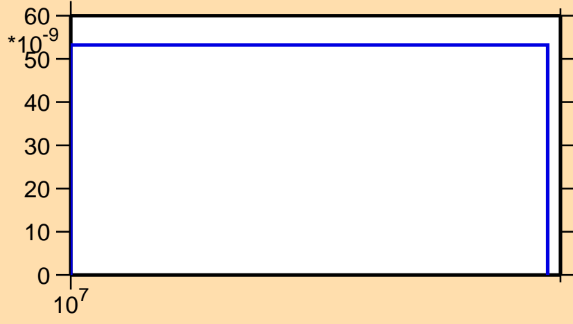
\sigma vs. E for ^{197}\text{Pb}(n,2np)
