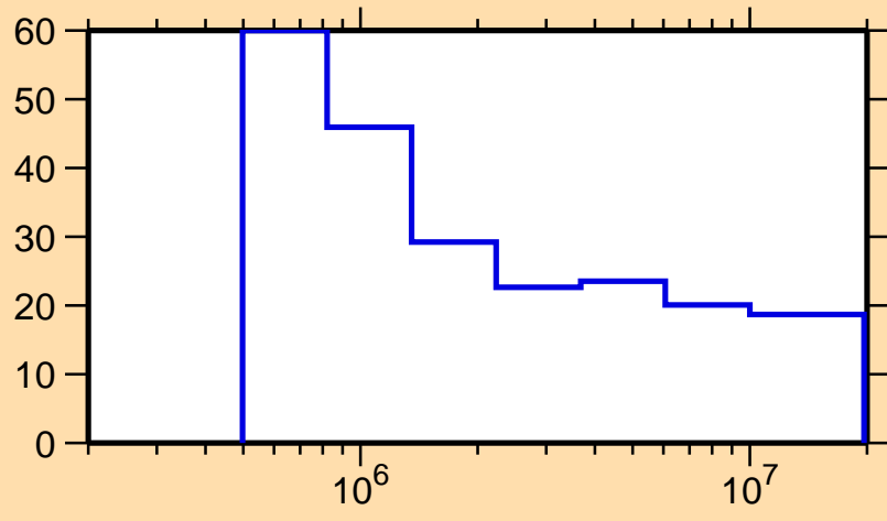
\Delta\sigma/\sigma vs. E for ^{197}\text{Pb}(n,\text{nonel.})
