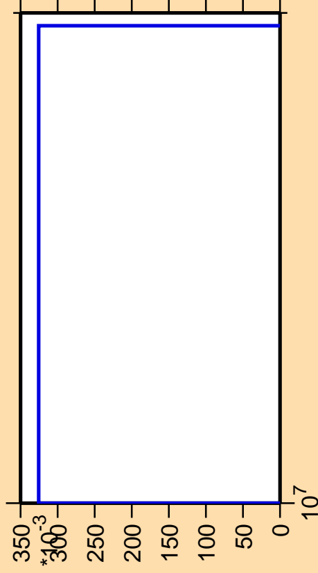
\Delta\sigma/\sigma vs. E for ^{197}\text{Pb}(\text{mt } 34)
