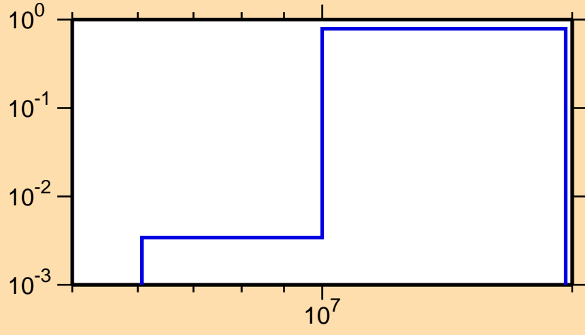
\sigma vs. E for ^{197}\text{Pb}(n,2n)
