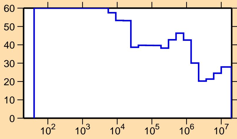
\Delta\sigma/\sigma vs. E for ^{197}\text{Pb}(n,\text{el.})
