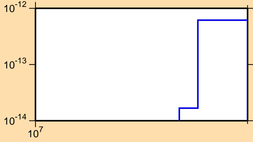
\sigma vs. E for ^{198}\text{Pb}(\text{mt } 45)
