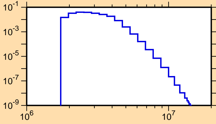
\sigma vs. E for ^{198}\text{Pb}(n,n_4)
