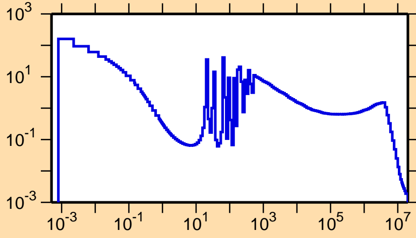
\sigma vs. E for ^{198}\text{Pb}(n,\gamma)
