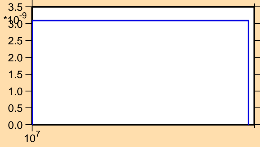
\sigma vs. E for ^{198}\text{Pb}(n,2np)
