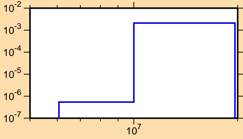
\sigma vs. E for ^{198}\text{Pb}(n,np)
