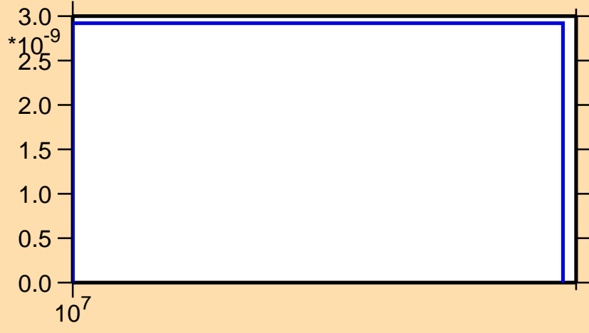
\sigma vs. E for ^{198}\text{Pb}(n,2n\alpha)
