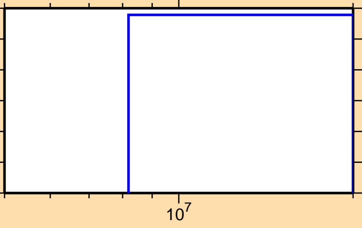
\sigma vs. E for ^{198}\text{Pb}(\text{mt } 45)
