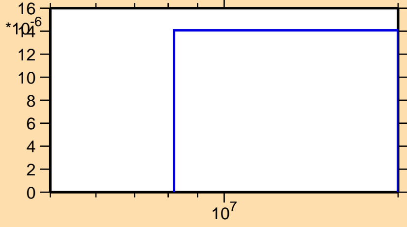
\sigma vs. E for ^{198}\text{Pb}(n,t)
