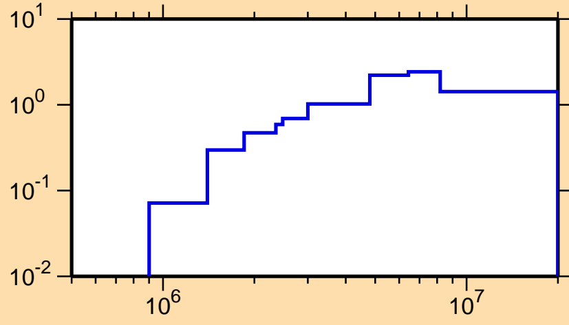
\sigma vs. E for ^{198}\text{Pb}(n,\text{inel.})
