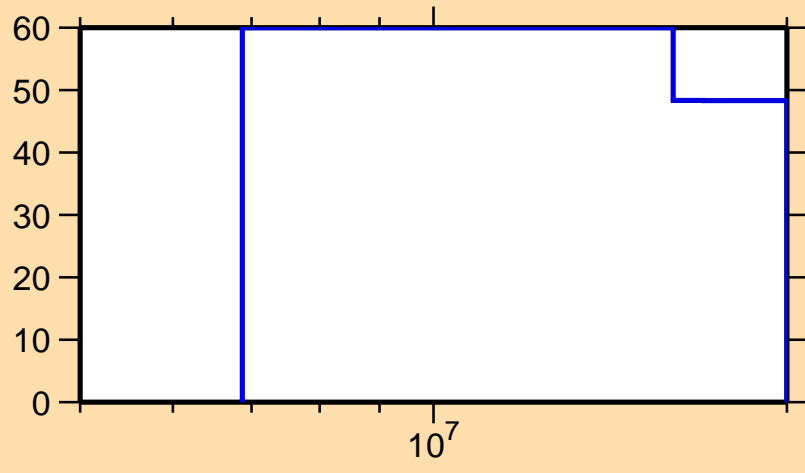
\Delta\sigma/\sigma vs. E for ^{199}\text{Pb}(n,2n)
