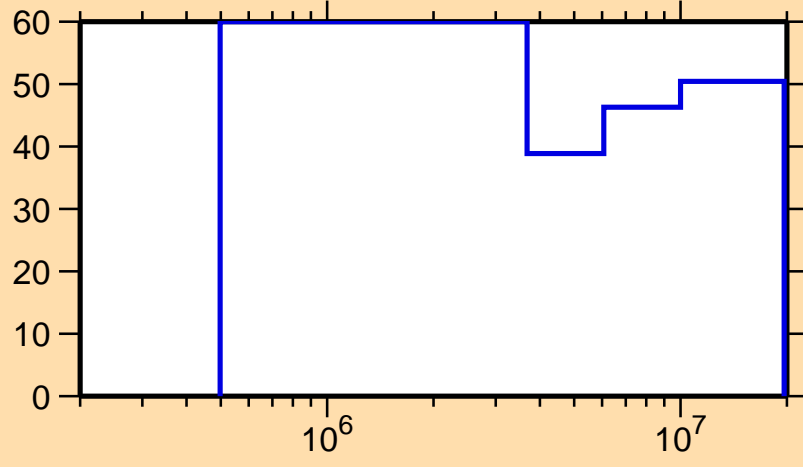
\Delta\sigma/\sigma vs. E for ^{199}\text{Pb}(n,n_1)
