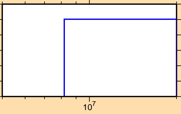
\sigma vs. E for ^{199}\text{Pb}(n,\text{pd})
