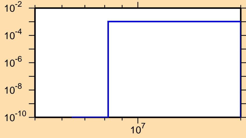
\sigma vs. E for ^{199}\text{Pb}(n,np)
