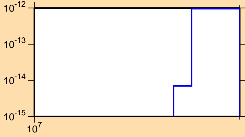
\sigma vs. E for ^{199}\text{Pb}(\text{mt } 34)
