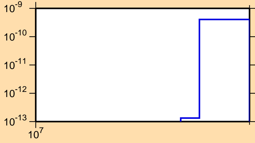
\sigma vs. E for ^{199}\text{Pb}(n,nt)
