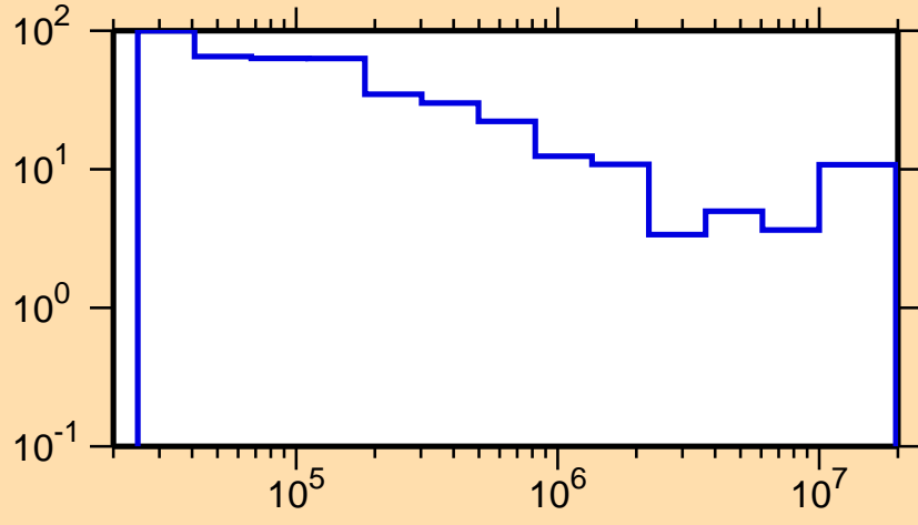
\Delta\sigma/\sigma vs. E for ^{199}\text{Pb}(n,n\text{cont.})
