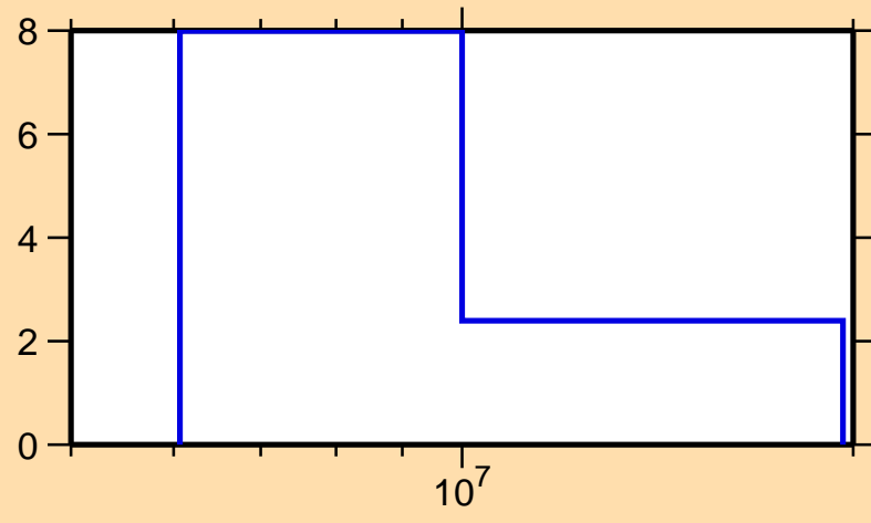
\Delta\sigma/\sigma vs. E for ^{199}\text{Pb}(n,\text{el.})
