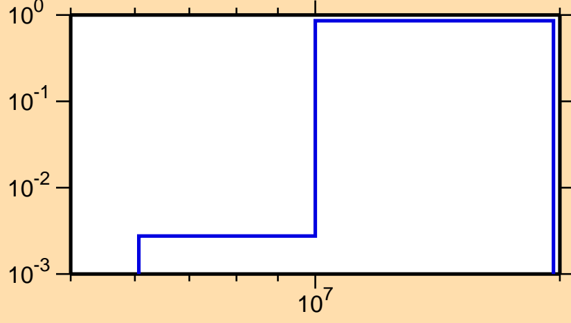
\sigma vs. E for ^{199}\text{Pb}(n,2n)
