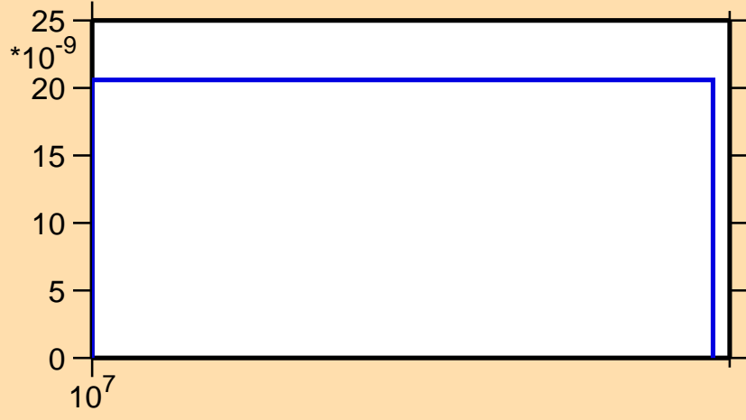
\sigma vs. E for ^{199}\text{Pb}(n,2np)
