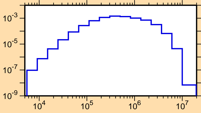
\sigma vs. E for ^{199}\text{Pb}(n,n_3)
