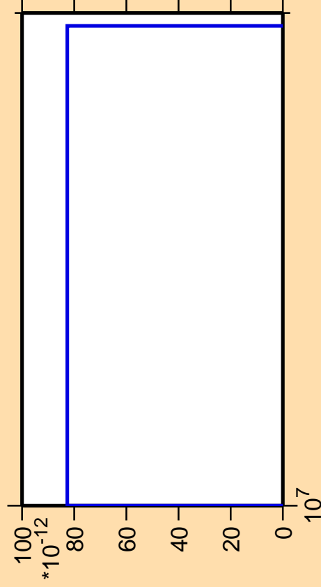
\Delta\sigma/\sigma vs. E for ^{199}\text{Pb} (mt 11)
