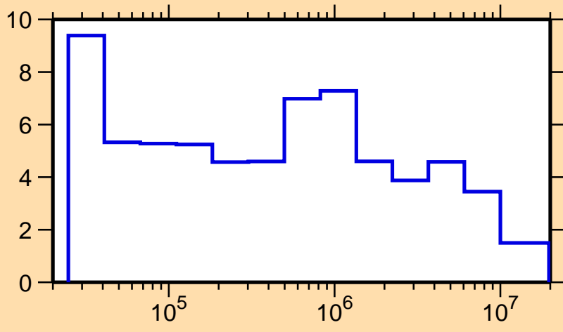
\Delta\sigma/\sigma vs. E for ^{199}\text{Pb}(n, \text{tot.})
