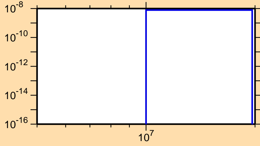
\sigma vs. E for ^{199}\text{Pb}(n,2n\alpha)
