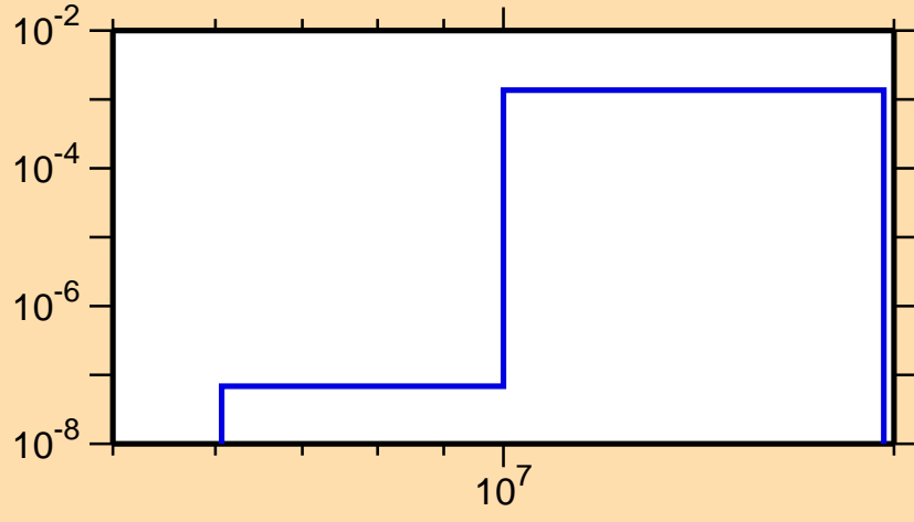
\sigma vs. E for ^{199}\text{Pb}(n,d)
