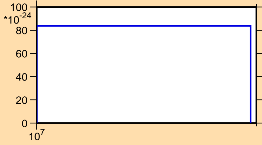
\sigma vs. E for ^{199}\text{Pb} (mt 11)
