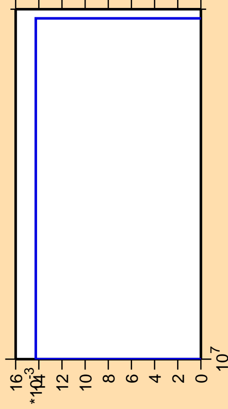
\Delta\sigma/\sigma vs. E for ^{199}\text{Pb}(n,\text{pt})
