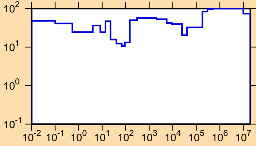
\Delta\sigma/\sigma vs. E for ^{199}\text{Pb}(n,\gamma)
