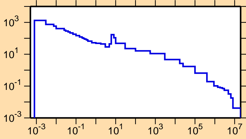
\sigma vs. E for ^{199}\text{Pb}(n,\gamma)
