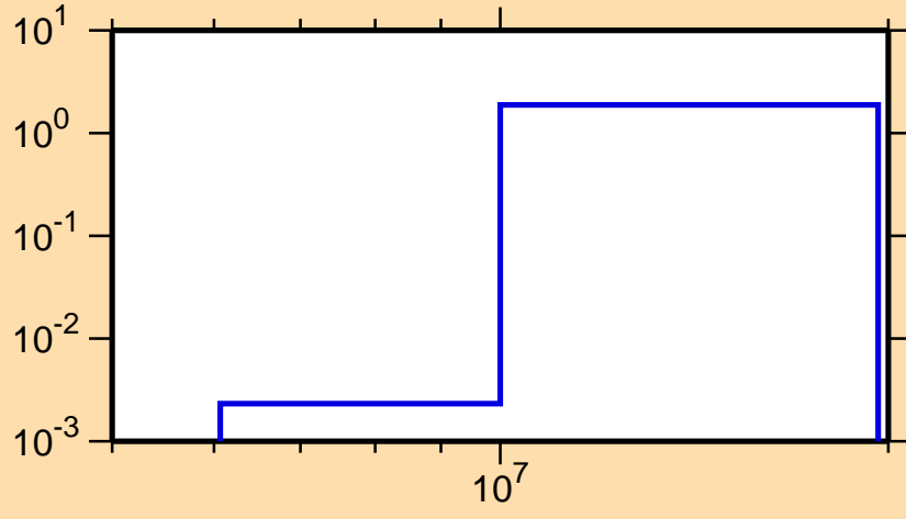
\sigma vs. E for ^{200}\text{Pb}(n,2n)
