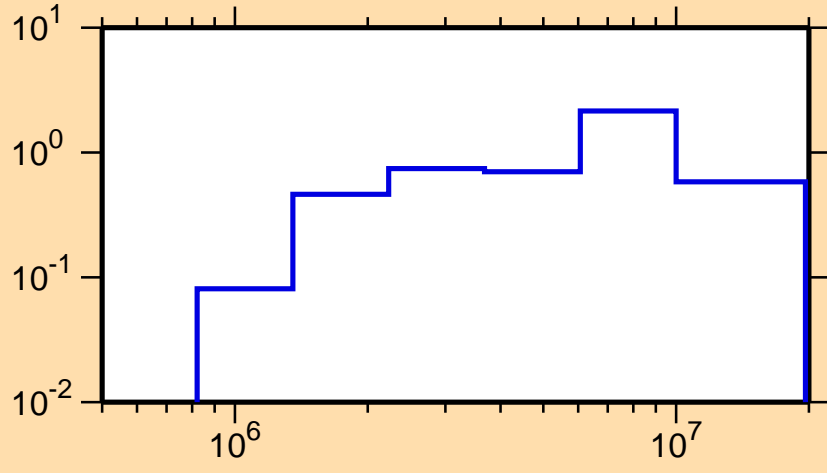
\sigma vs. E for ^{200}\text{Pb}(n,\text{inel.})
