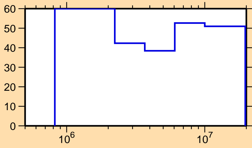
\Delta\sigma/\sigma vs. E for ^{200}\text{Pb}(n,n_1)
