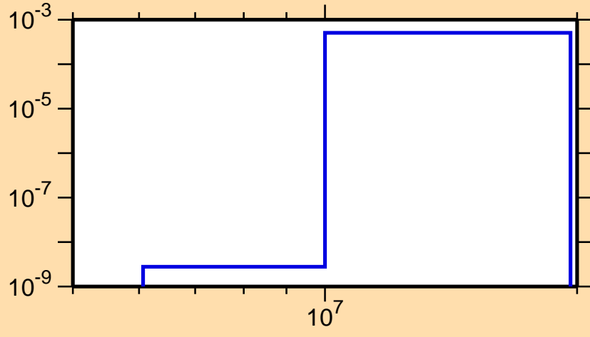
\sigma vs. E for ^{200}\text{Pb}(n,d)
