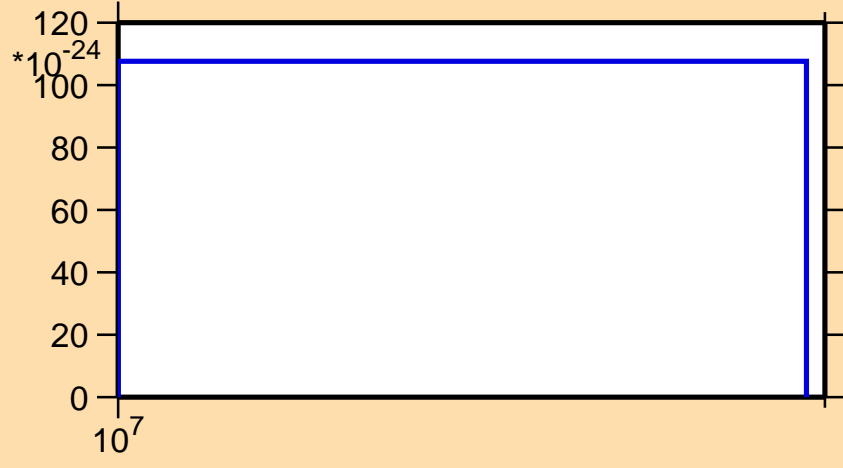
\sigma vs. E for ^{200}\text{Pb} (mt 11)
