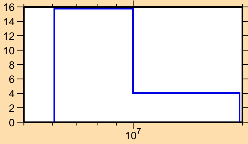
\Delta\sigma/\sigma vs. E for ^{200}\text{Pb}(n,\text{tot.})
