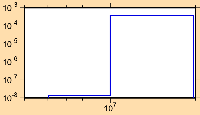
\sigma vs. E for ^{200}\text{Pb}(n,np)
