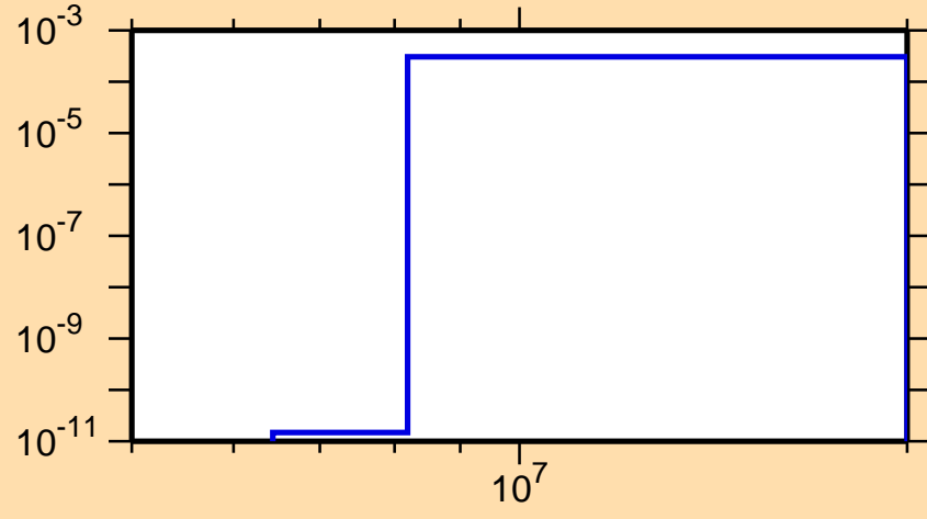
\sigma vs. E for ^{200}\text{Pb}(n,np)
