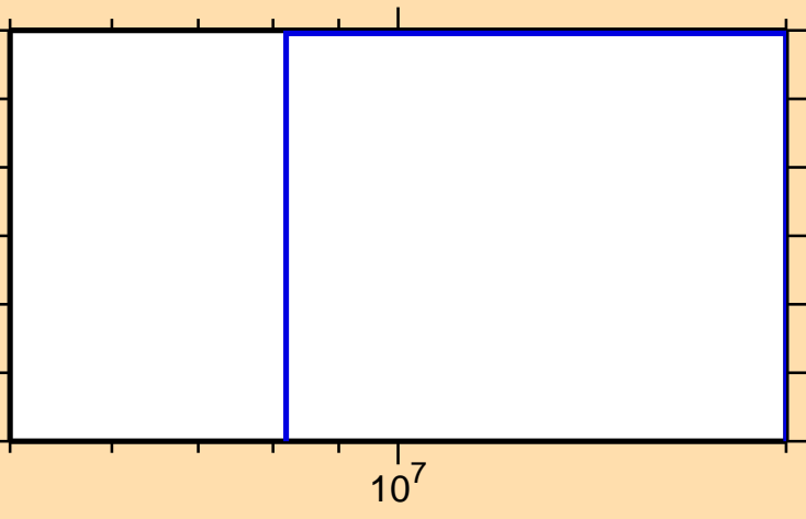
\sigma vs. E for ^{200}\text{Pb}(n,\text{pd})
