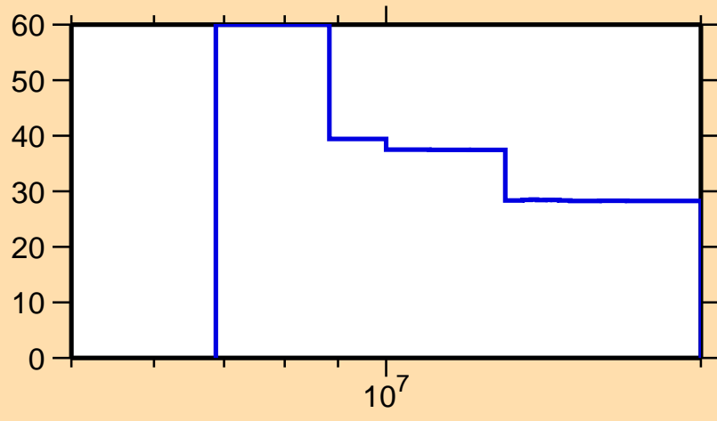
\Delta\sigma/\sigma vs. E for ^{201}\text{Pb}(n,2n)
