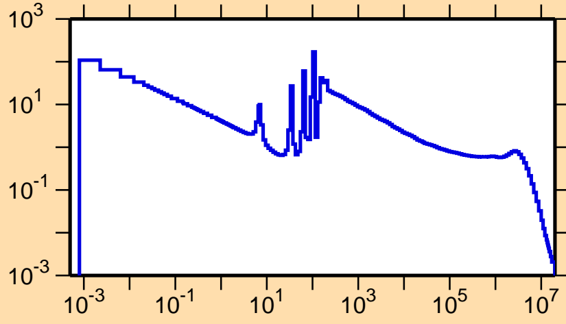
\sigma vs. E for ^{201}\text{Pb}(n,\gamma)
