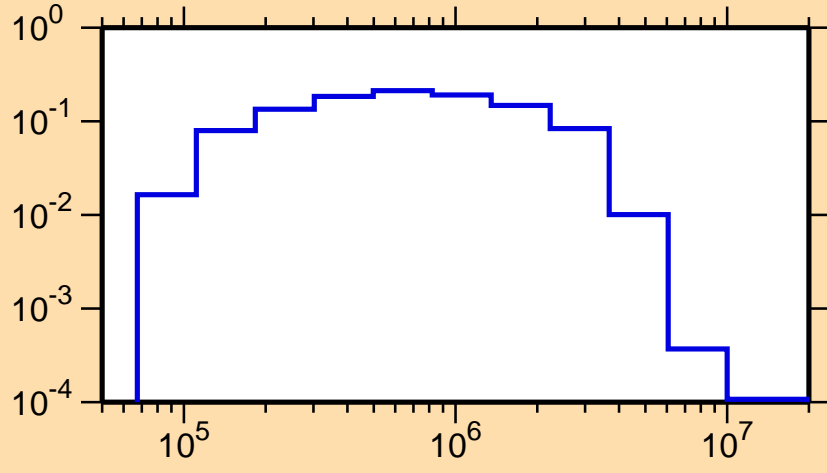
\sigma vs. E for ^{201}\text{Pb}(n,n_1)
