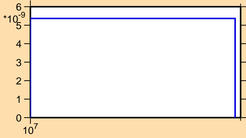
\sigma vs. E for ^{201}\text{Pb}(n,2np)
