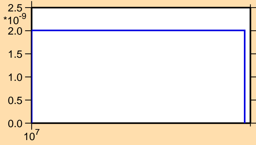
\sigma vs. E for ^{201}\text{Pb}(n,2n\alpha)
