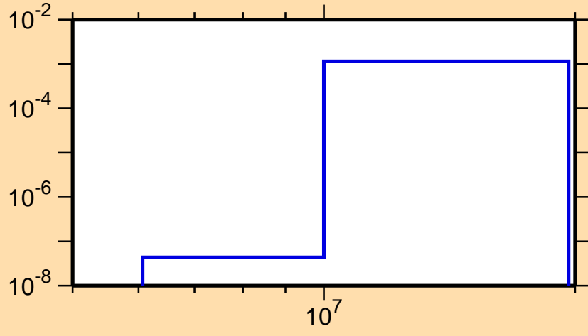
\sigma vs. E for ^{201}\text{Pb}(n,d)
