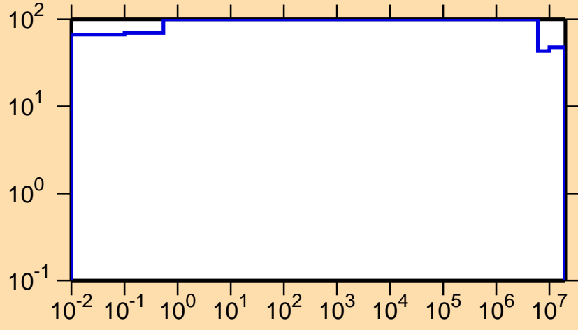
\Delta\sigma/\sigma vs. E for ^{201}\text{Pb}(n,p)
