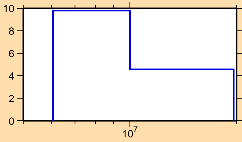
\Delta\sigma/\sigma vs. E for ^{201}\text{Pb}(n,\text{tot.})
