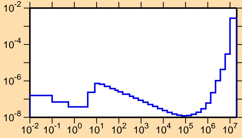
\sigma vs. E for ^{201}\text{Pb}(n,\alpha)
