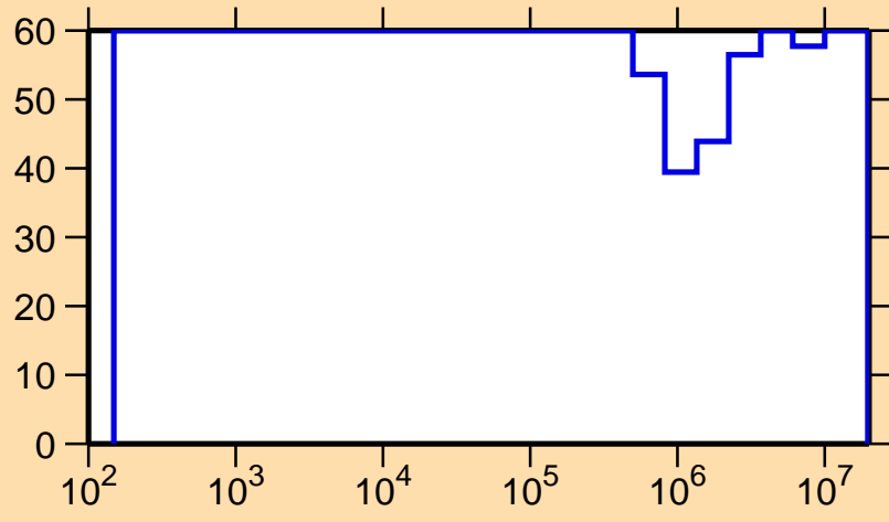
\Delta\sigma/\sigma vs. E for ^{201}\text{Pb}(n,n_1)
