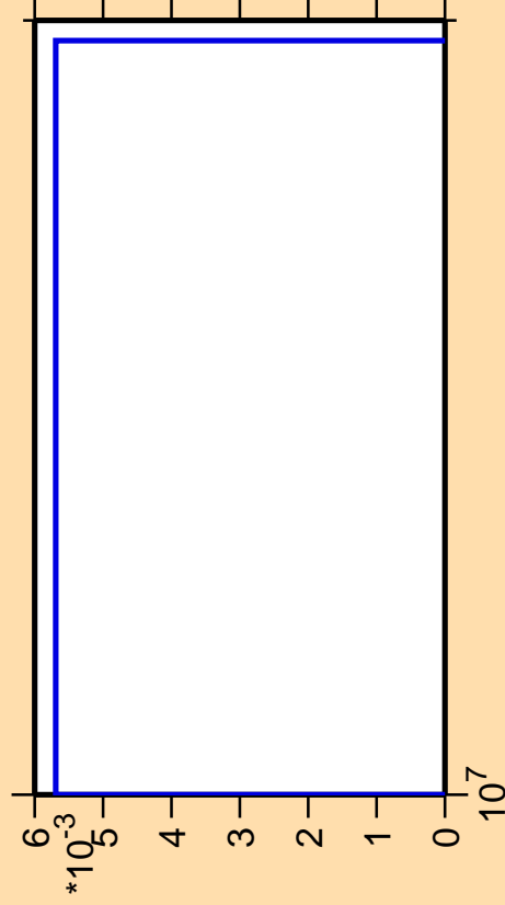
\Delta\sigma/\sigma vs. E for ^{201}\text{Pb} (mt 34)
