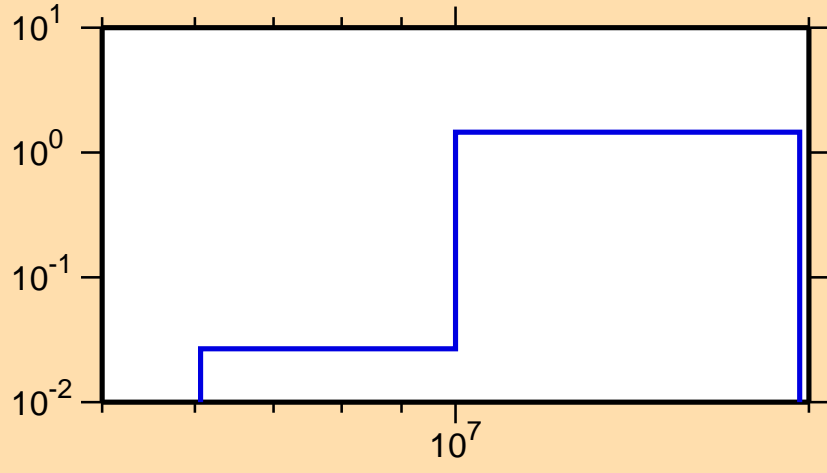
\sigma vs. E for ^{201}\text{Pb}(n,2n)
