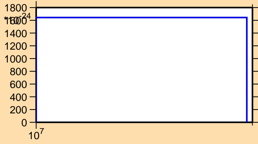
\sigma vs. E for ^{201}\text{Pb} (mt 11)
