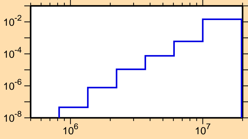
\sigma vs. E for ^{201}\text{Pb}(n,p)
