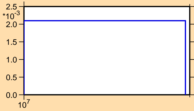
\sigma vs. E for ^{201}\text{Pb}(n,3n)
