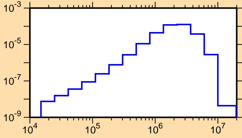
\sigma vs. E for ^{202}\text{Pb}(n,n_4)
