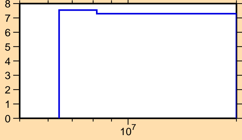
\Delta\sigma/\sigma vs. E for ^{202}\text{Pb}(n,\text{el.})
