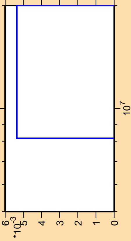
\Delta\sigma/\sigma vs. E for ^{202}\text{Pb}(n,pd)
