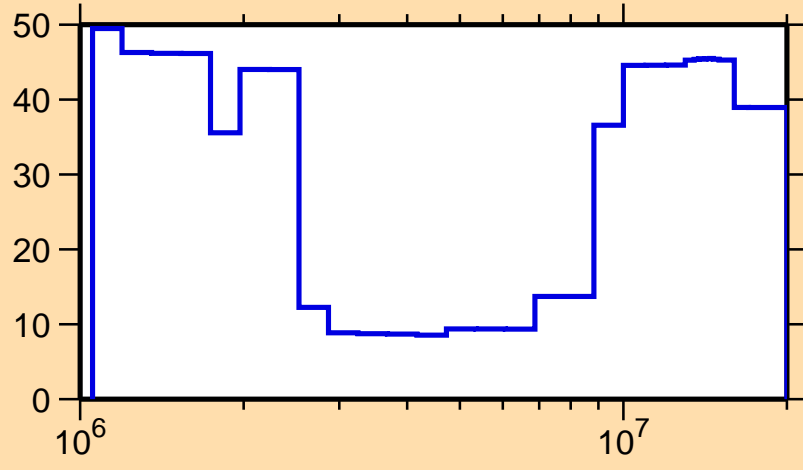
\Delta\sigma/\sigma vs. E for ^{203}\text{Pb}(n,n\text{cont.})
