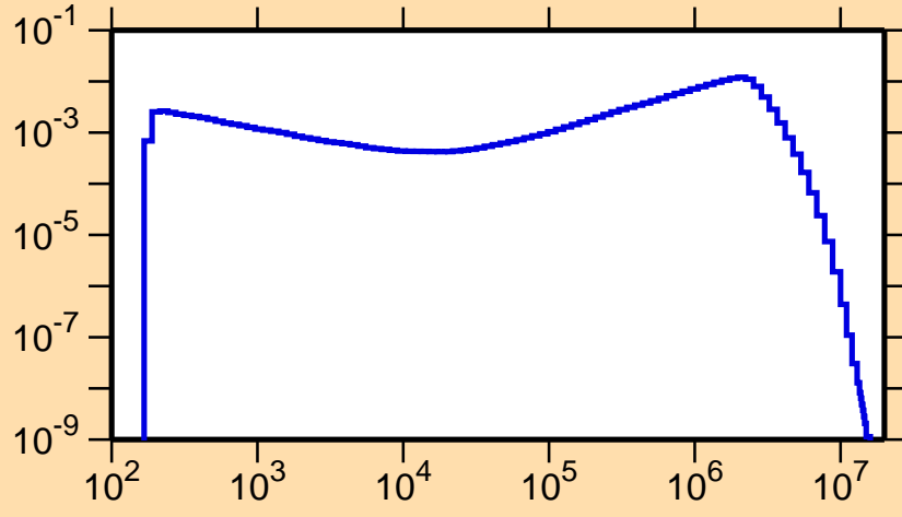
\sigma vs. E for ^{203}\text{Pb}(n,n_3)
