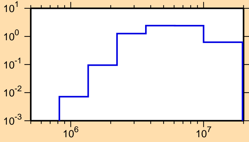
\sigma vs. E for ^{203}\text{Pb}(n,n\text{cont.})
