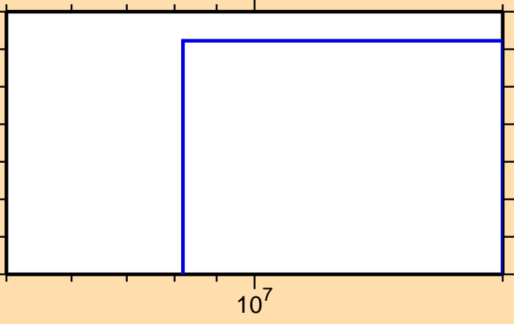
\sigma vs. E for ^{203}\text{Pb}(n,2n\alpha)
