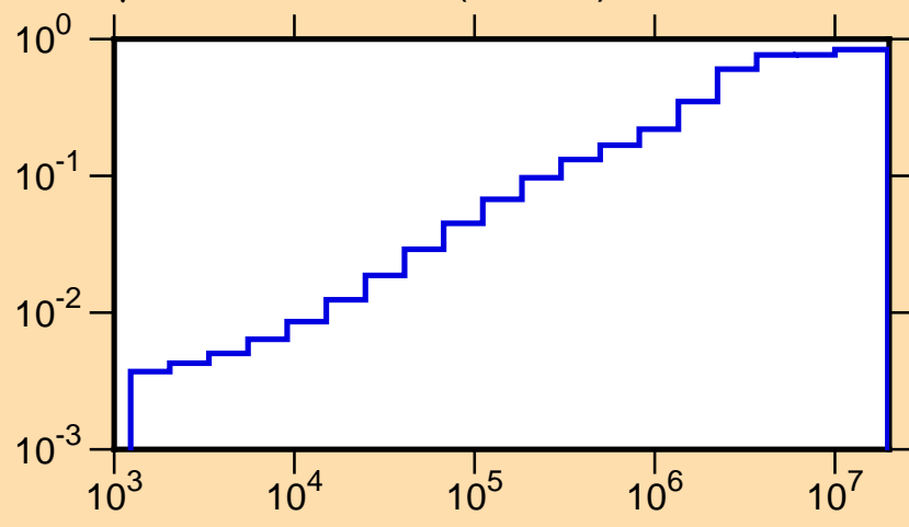
\mu vs. E for ^{204}\text{Pb}(\text{mt251})
