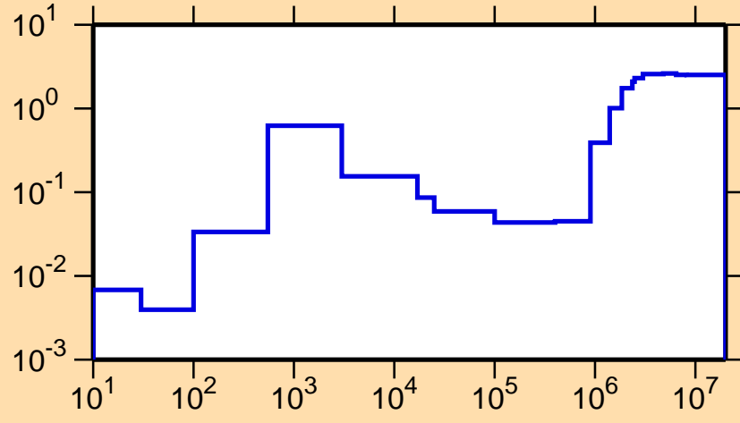
\sigma vs. E for ^{204}\text{Pb}(n,\text{nonel.})
