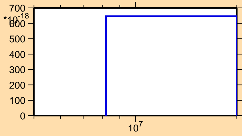
\sigma vs. E for ^{204}\text{Pb}(n,p\alpha)
