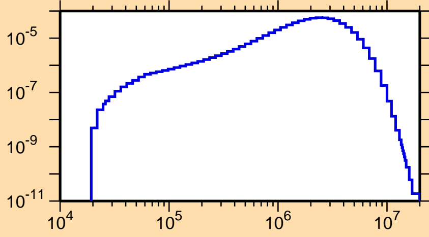
\sigma vs. E for ^{204}\text{Pb}(n,n_1)
