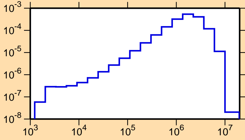
\sigma vs. E for ^{204}\text{Pb}(n,n_4)
