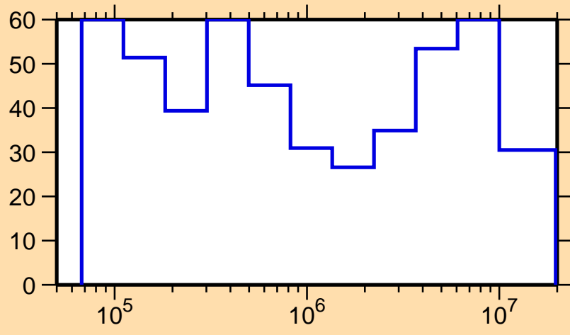
\Delta\sigma/\sigma vs. E for ^{204}\text{Pb}(n,n_1)
