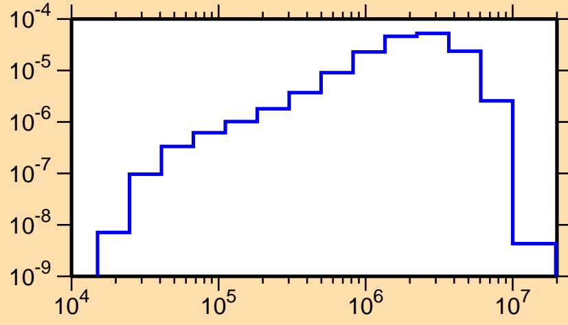
\sigma vs. E for ^{204}\text{Pb}(n,n_1)
