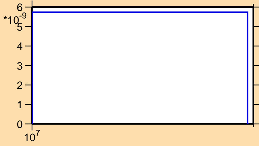
\sigma vs. E for ^{204}\text{Pb}(n,2np)
