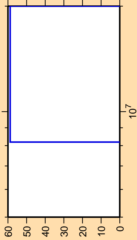
\Delta\sigma/\sigma vs. E for ^{204}\text{Pb}(n,nd)
