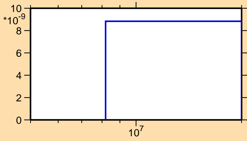
\sigma vs. E for ^{204}\text{Pb}(n,nd)
