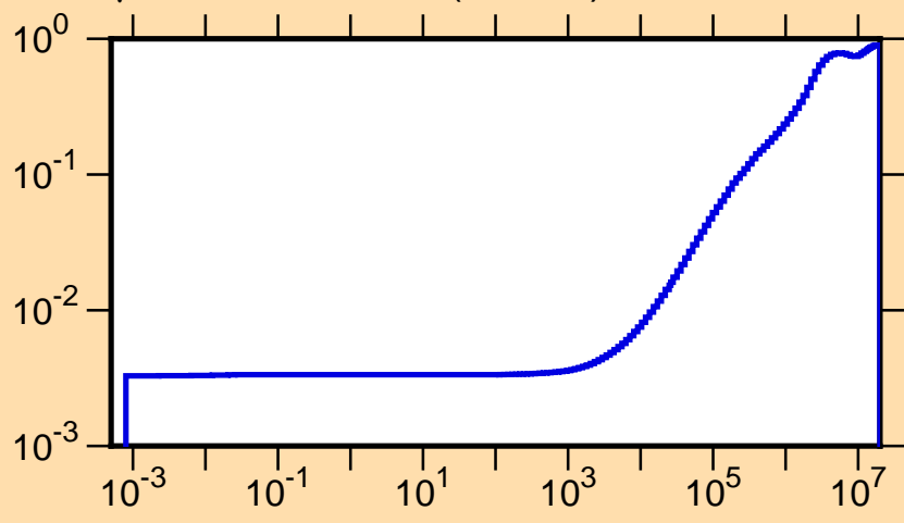
\mu vs. E for ^{205}\text{Pb}(\text{mt251})
