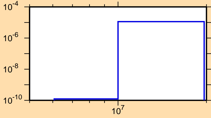
\sigma vs. E for ^{205}\text{Pb}(n,n\alpha)
