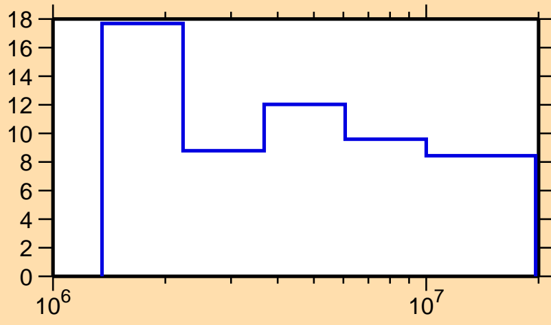
\Delta\sigma/\sigma vs. E for ^{205}\text{Pb}(n, el.)
