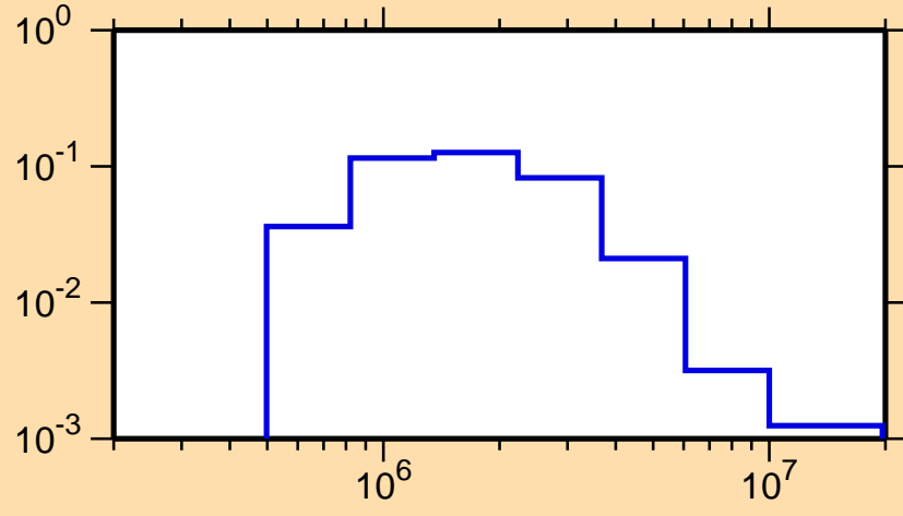
\sigma vs. E for ^{205}\text{Pb}(n,n_3)
