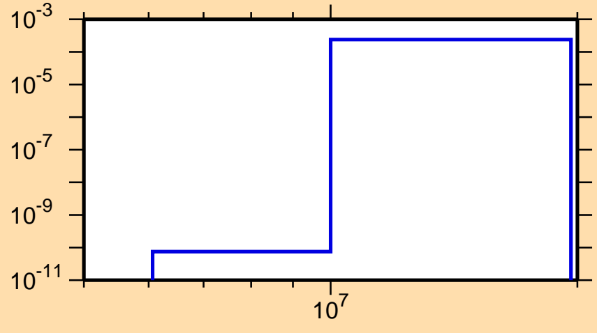
\sigma vs. E for ^{205}\text{Pb}(n,d)
