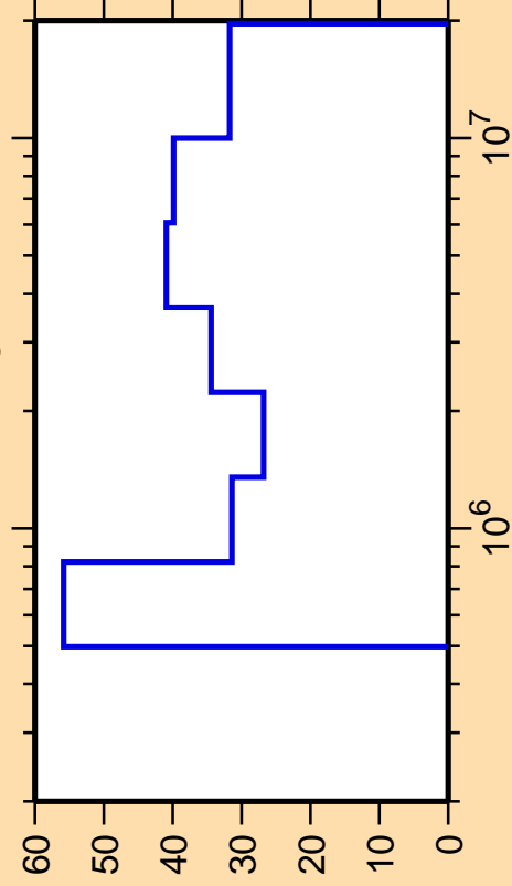
\Delta\sigma/\sigma vs. E for ^{205}\text{Pb}(n,n_3)
