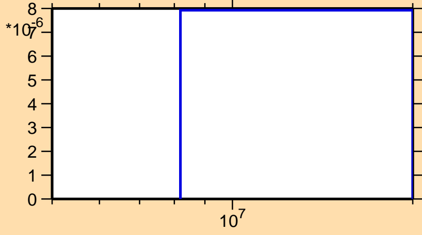
\sigma vs. E for ^{207}\text{Pb}(n,t)
