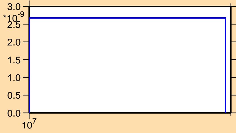
\sigma vs. E for ^{209}\text{Pb}(n,2n\alpha)
