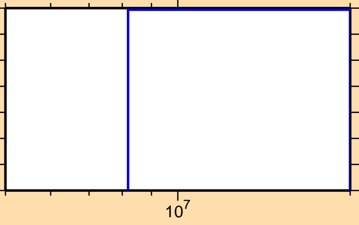
\sigma vs. E for ^{209}\text{Pb}(n,\text{nd})
