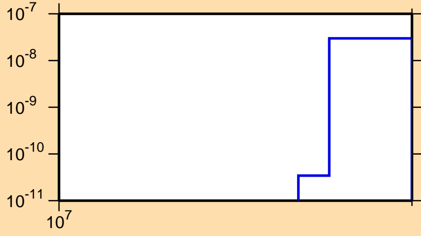
\sigma vs. E for ^{210}\text{Pb}(n,2np)
