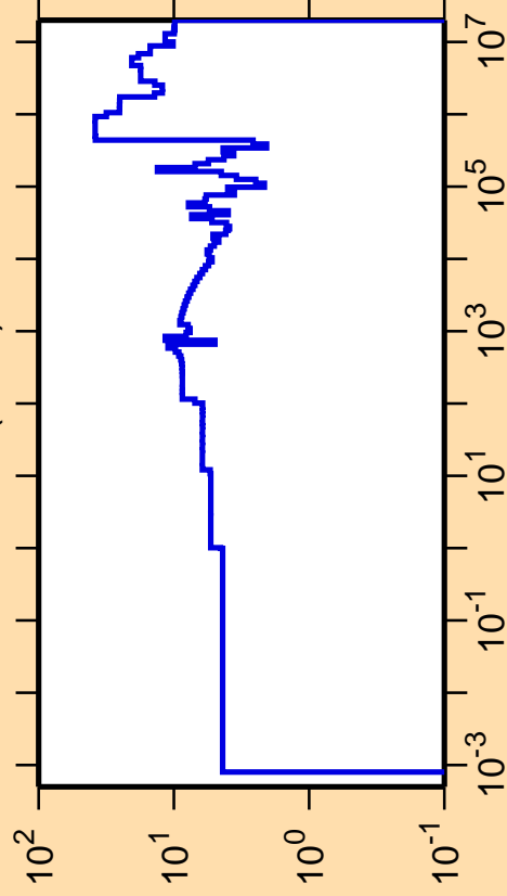
\Delta\sigma/\sigma vs. E for ^{210}\text{Pb}(n,\text{el.})
