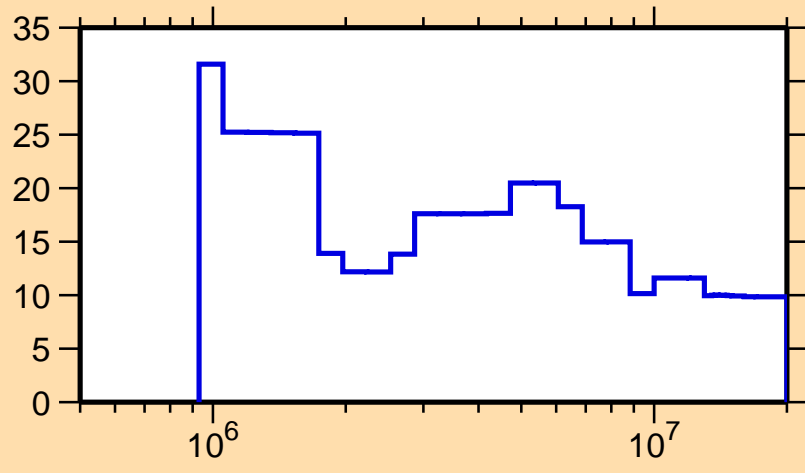
\Delta\sigma/\sigma vs. E for ^{210}\text{Pb}(n,\text{el.})
