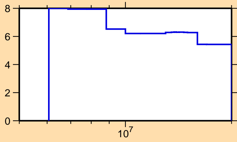
\Delta\sigma/\sigma vs. E for ^{210}\text{Pb}(n,\text{nonel.})
