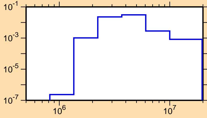
\sigma vs. E for ^{210}\text{Pb}(n,n_4)
