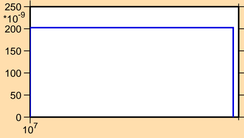
\sigma vs. E for ^{210}\text{Pb}(n,nt)
