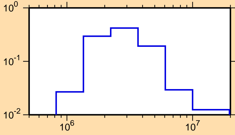
\sigma vs. E for ^{210}\text{Pb}(n,n_2)
