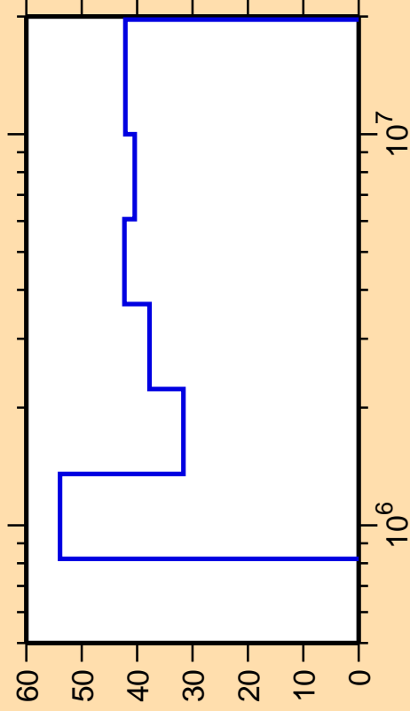
\Delta\sigma/\sigma vs. E for ^{210}\text{Pb}(n,n_2)
