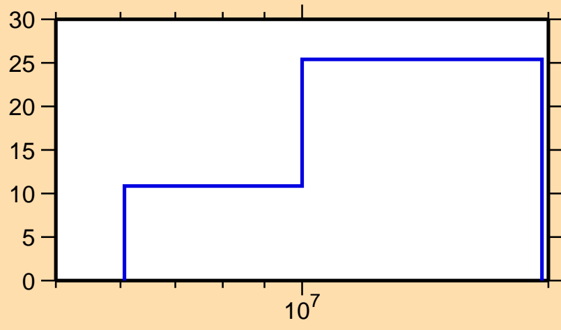
\Delta\sigma/\sigma vs. E for ^{210}\text{Pb}(n,2n)
