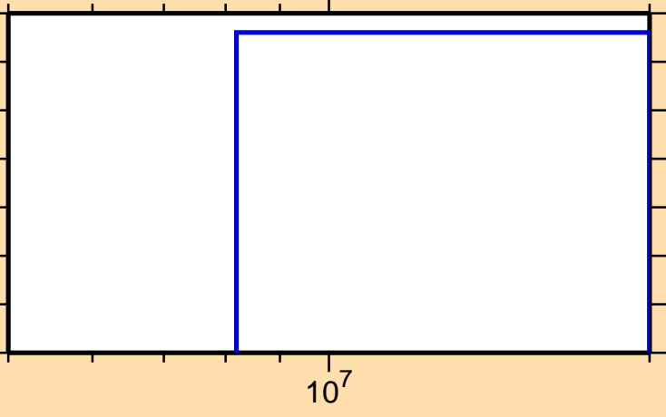
\sigma vs. E for ^{210}\text{Pb}(n,d)
