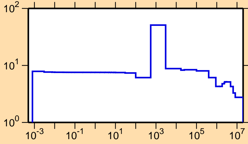
\sigma vs. E for ^{210}\text{Pb}(n,\text{el.})
