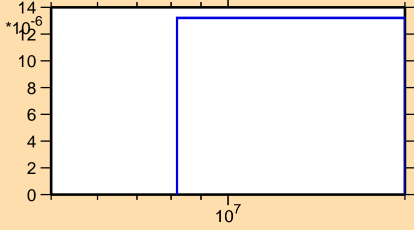
\sigma vs. E for ^{210}\text{Pb}(n,d)
