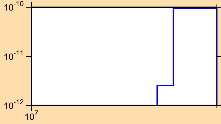
\sigma vs. E for ^{211}\text{Pb}(n,p\alpha)
