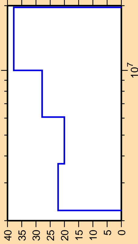
\Delta\sigma/\sigma vs. E for ^{211}\text{Pb}(n,n\text{cont.})
