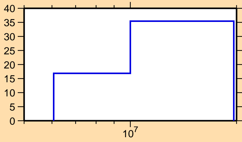
\Delta\sigma/\sigma vs. E for ^{211}\text{Pb}(n,2n)
