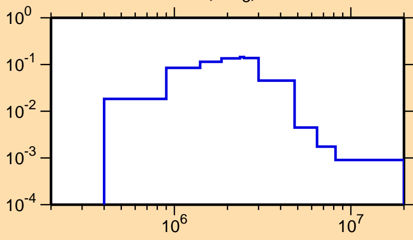
\sigma vs. E for ^{211}\text{Pb}(n,n_3)
