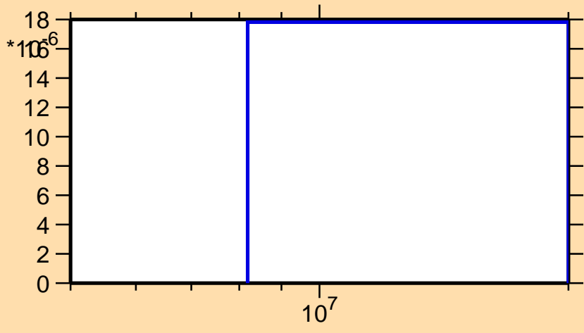
\sigma vs. E for ^{211}\text{Pb}(n,d)
