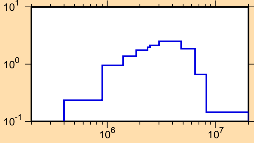
\sigma vs. E for ^{211}\text{Pb}(n,\text{inel.})
