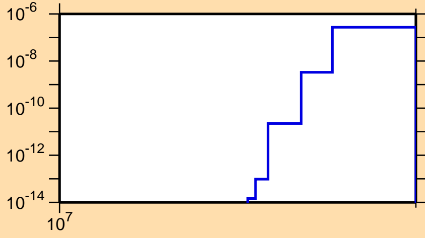
\sigma vs. E for ^{212}\text{Pb}(n,nd)
