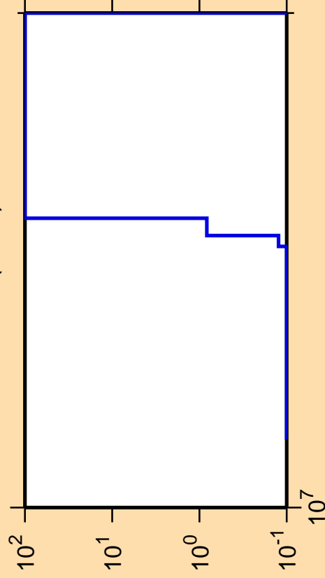
\Delta\sigma/\sigma vs. E for ^{212}\text{Pb}(n,nd)
