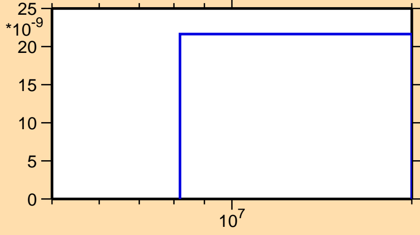
\sigma vs. E for ^{212}\text{Pb}(n,2n\alpha)
