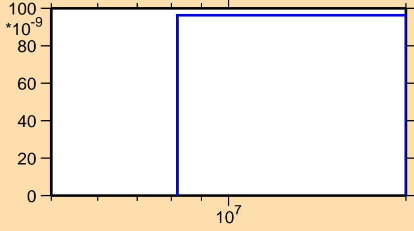
\sigma vs. E for ^{212}\text{Pb}(n,nt)
