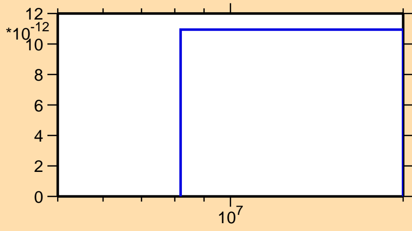
\sigma vs. E for ^{212}\text{Pb}(n,3n\alpha)
