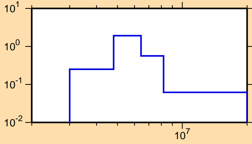
\sigma vs. E for ^{212}\text{Pb}(n,n\text{cont.})
