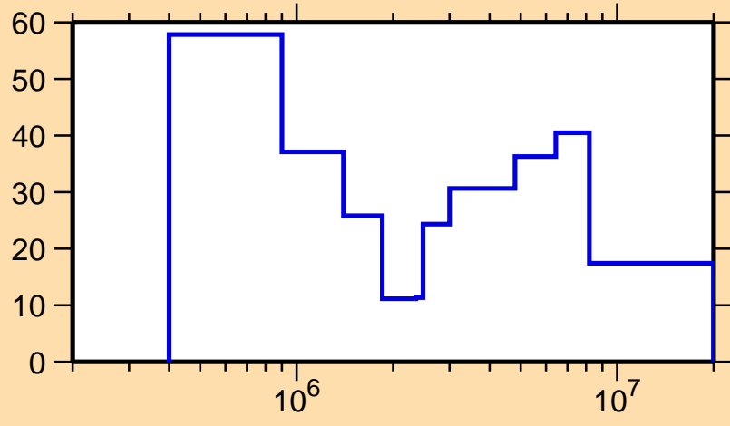
\Delta\sigma/\sigma vs. E for ^{212}\text{Pb}(n,\text{el.})
