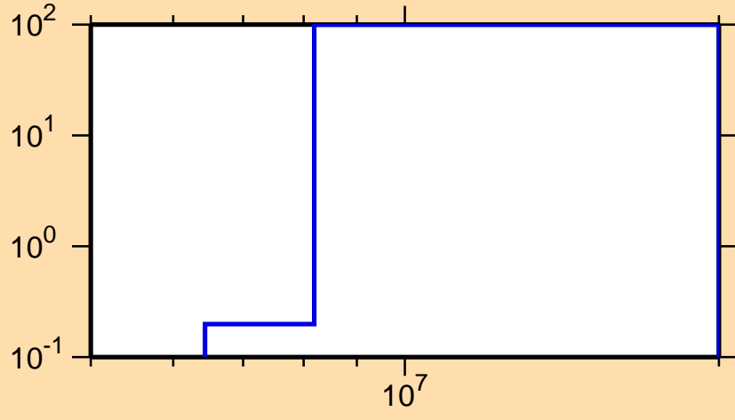
\Delta\sigma/\sigma vs. E for ^{212}\text{Pb}(n,p)
