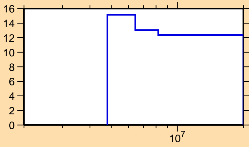
\Delta\sigma/\sigma vs. E for ^{212}\text{Pb}(n,\text{nonel.})
