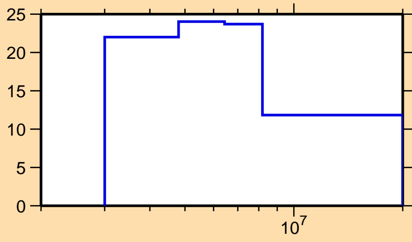
\Delta\sigma/\sigma vs. E for ^{212}\text{Pb}(n, \text{tot.})
