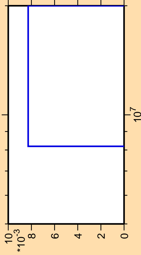
\Delta\sigma/\sigma vs. E for ^{212}\text{Pb} (mt 11)
