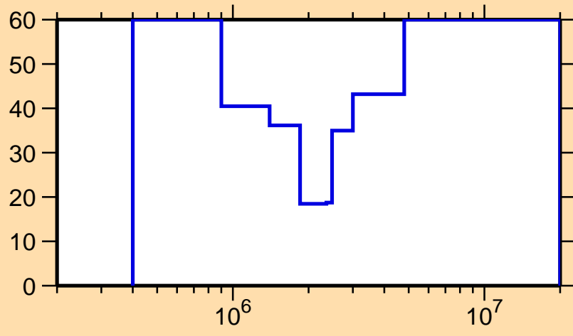
\Delta\sigma/\sigma vs. E for ^{212}\text{Pb}(n,n_1)
