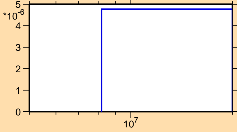
\sigma vs. E for ^{212}\text{Pb}(n,np)
