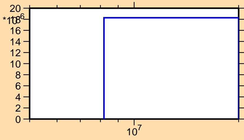
\sigma vs. E for ^{212}\text{Pb}(n,t)
