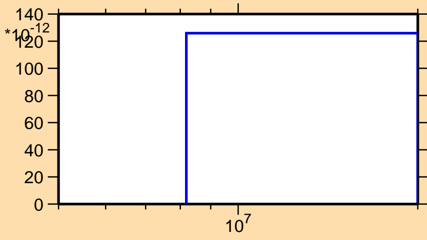
\sigma vs. E for ^{212}\text{Pb}(n,2np)
