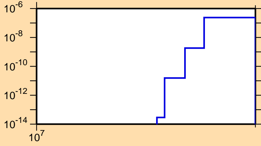
\sigma vs. E for ^{213}\text{Pb}(n,2np)
